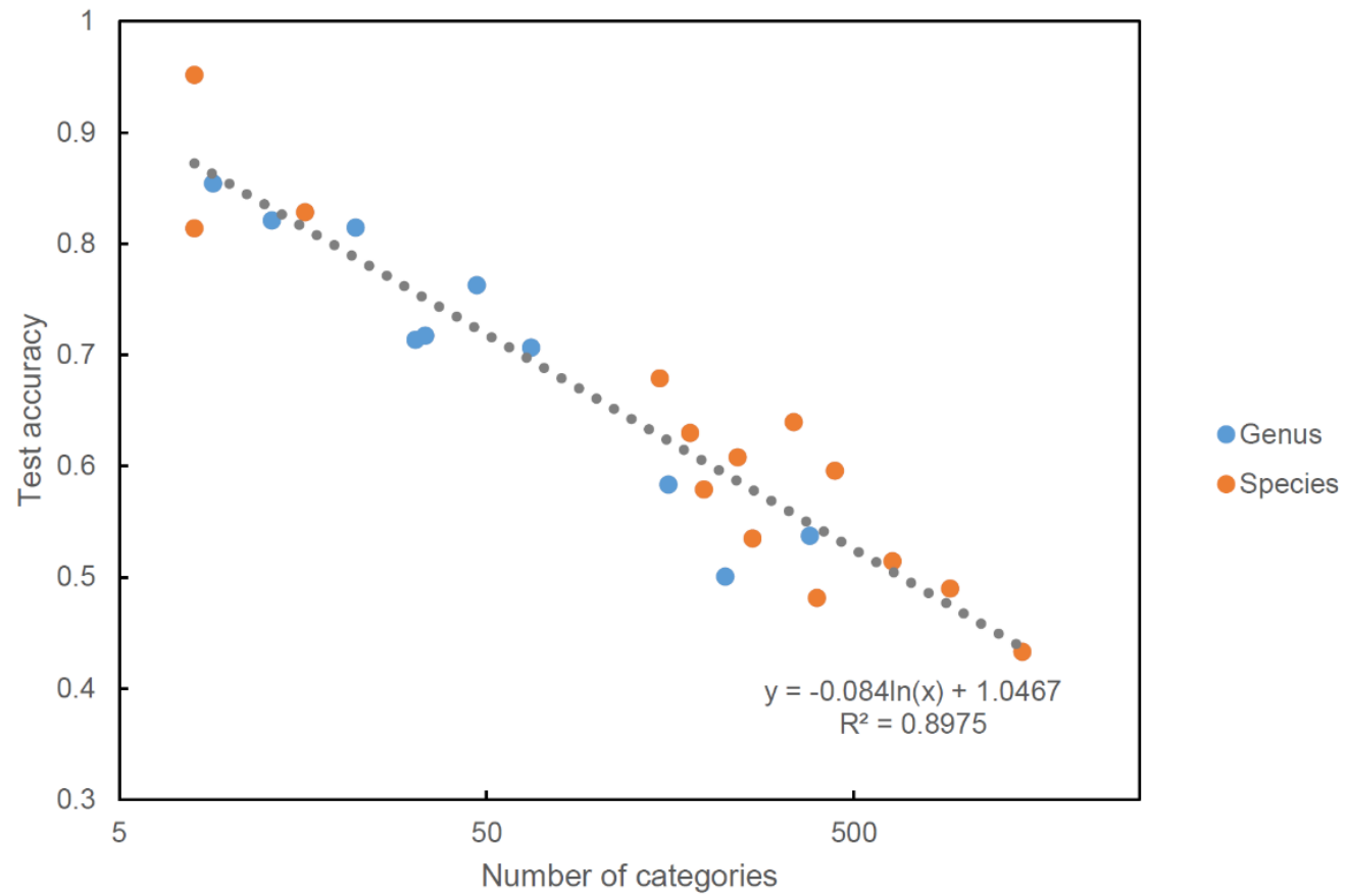
Appendix S4. Relationship between the number of categories and the accuracy. The two correspond well to the logarithmic relationship.
