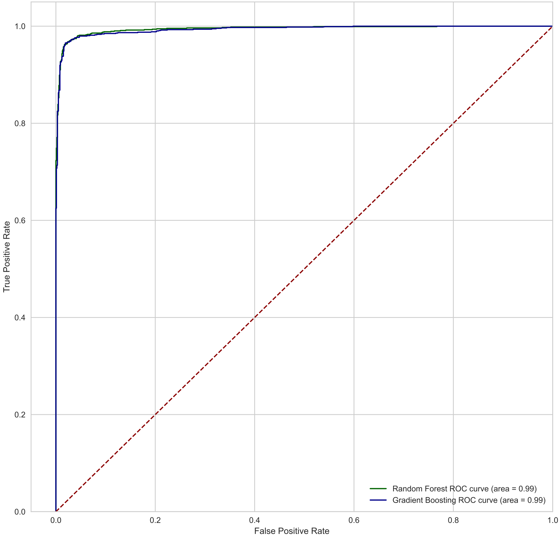
ROC curve: Random Forest and Gradient Boosting Models
