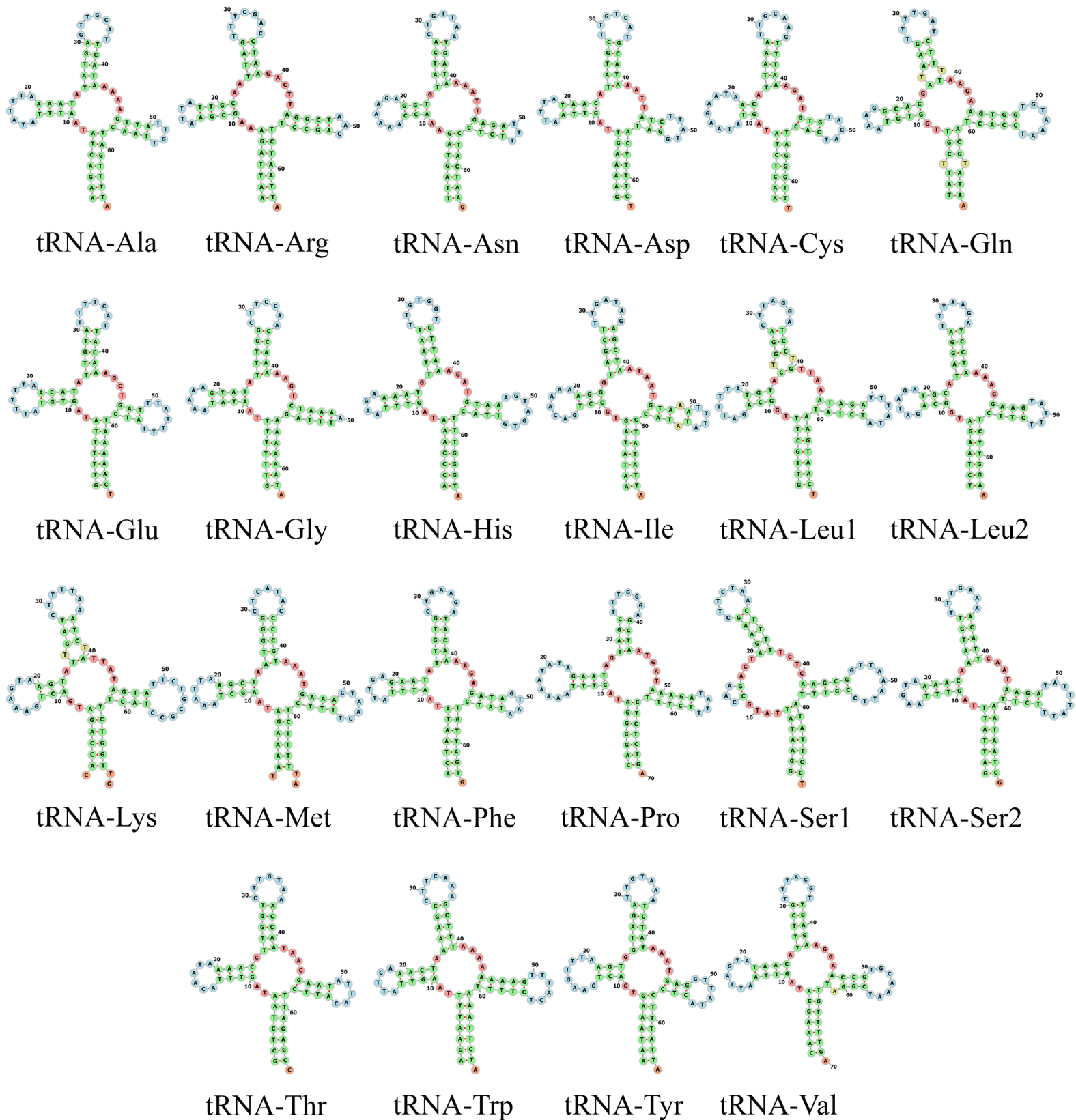
D) Secondary structures of 22 transfer RNA genes in Hapalocarcinus marsupialis s.l.
