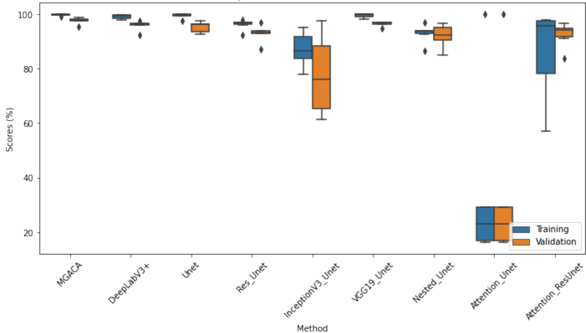
Comparison of all models Performance
