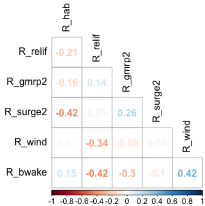
Figure S4: Pairwise comparisons and correlation scores of six variables in the exposure index.
