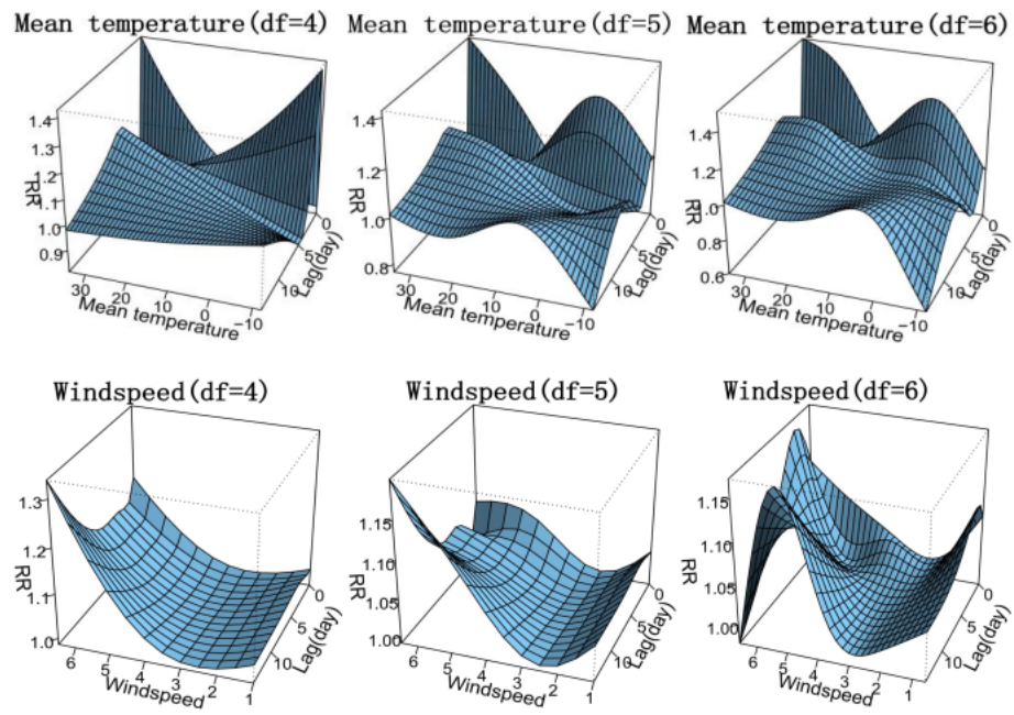
Fig.S2 Sensitivity analysis results of air pollution after changing the degree of freedom of time term
