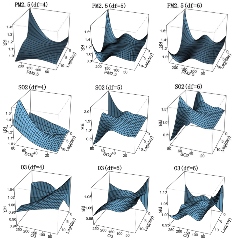
Fig.S3 Sensitivity analysis results after changing the degree of freedom of each air pollution
