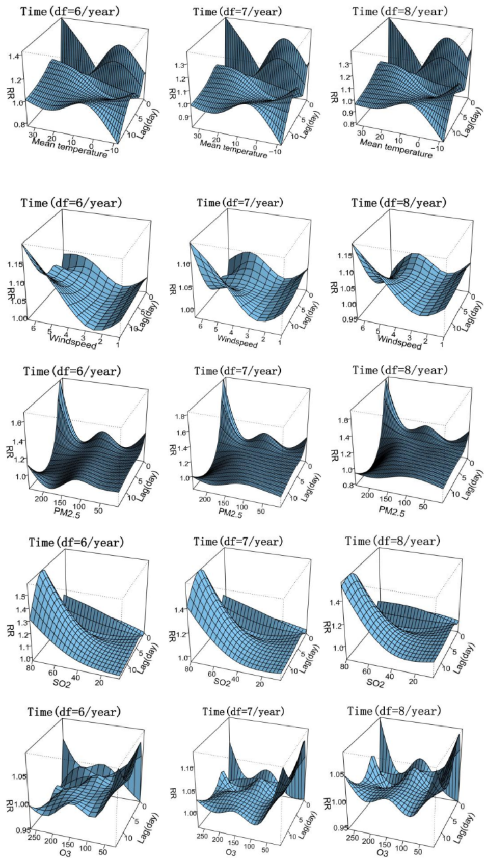
Fig.S1 Sensitivity analysis results of meteorological factors and air pollutions after changing the degree of freedom of time term
