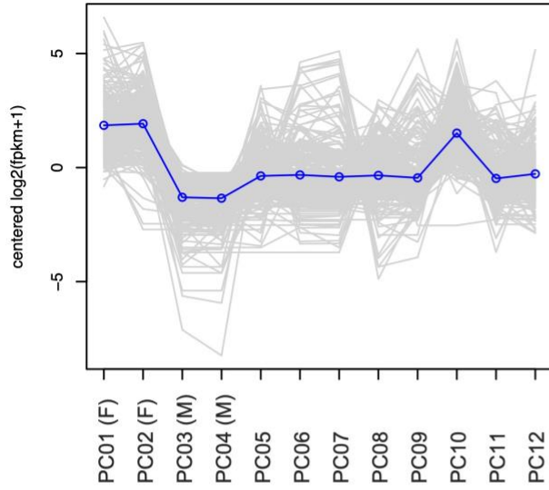
Subcluster I (283 transcripts)
