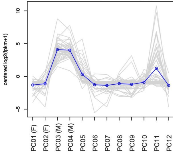
Subcluster III (46 transcripts)
