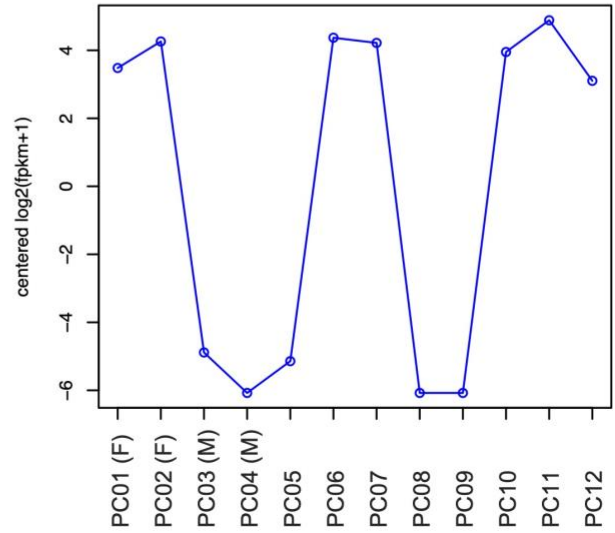
Subcluster IV (1 transcript)
