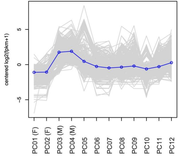
Subcluster II (525 transcripts)
