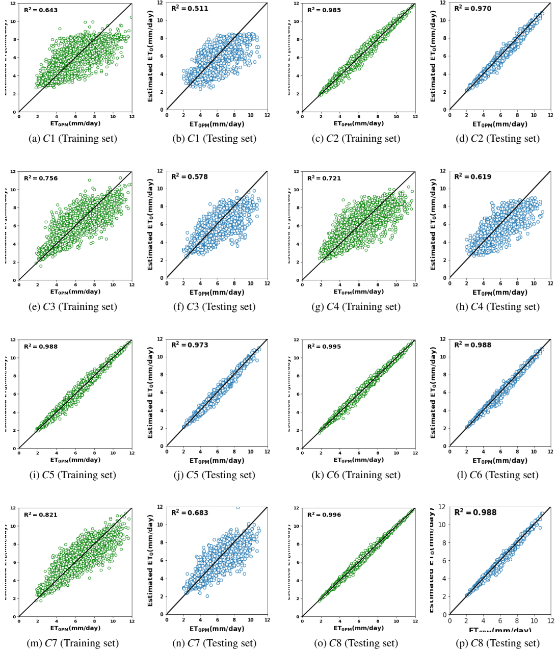
Figure 10: Scatter plots of estimated ET_0 against ET_{0PM} obtained for the training and testing sets of Berubari
