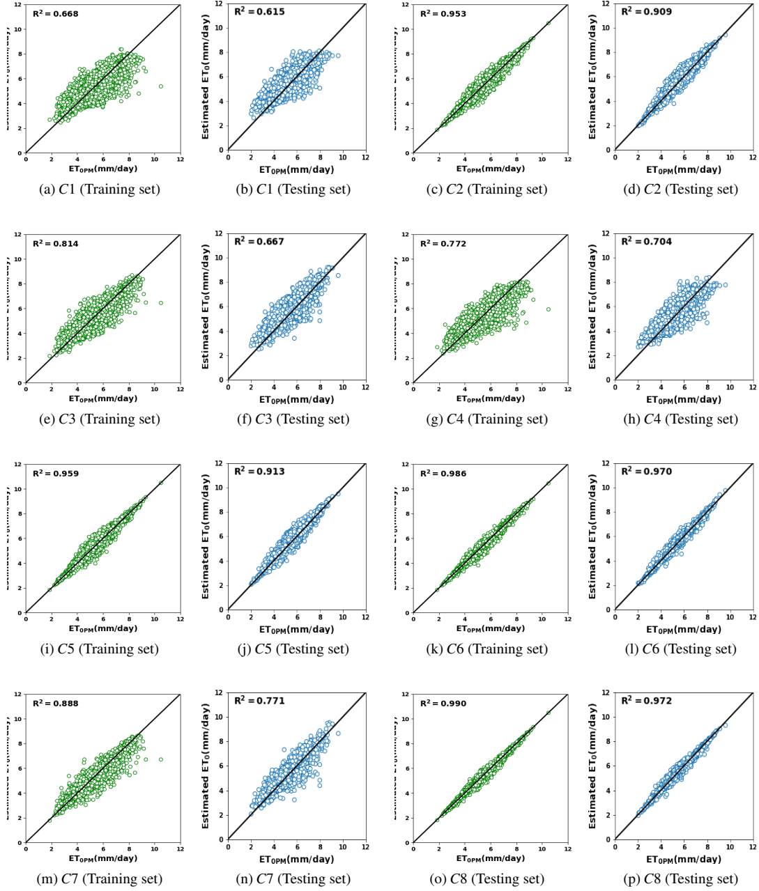
Figure 14: Scatter plots of estimated ET_0 against ET_{0PM} obtained for the training and testing sets of Jayanti
