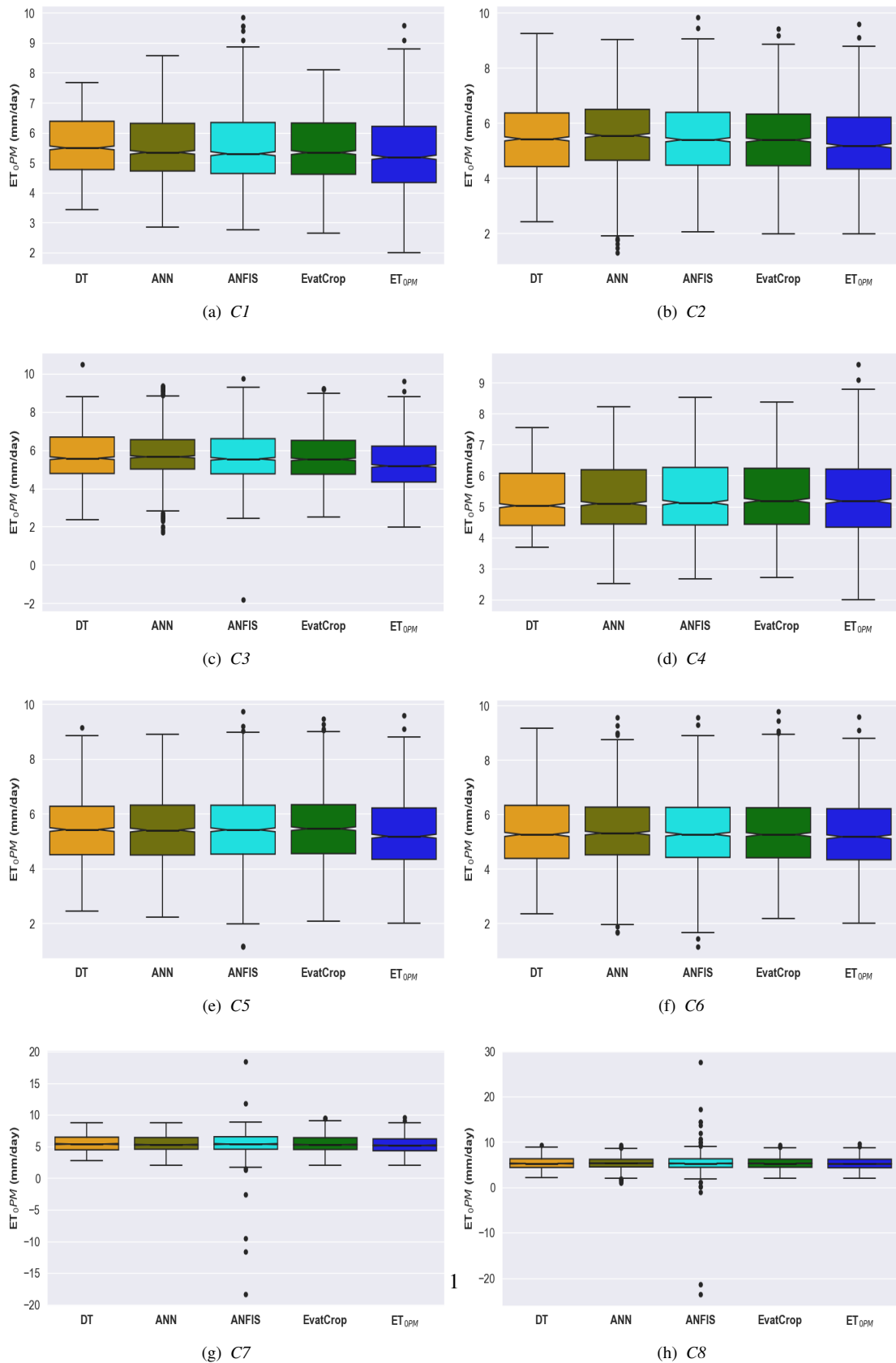
Figure 15: Boxplots for estimated ET_0 of DT, ANN, ANFIS, EvatCrop , and ET_{0PM} obtained for the testing set of Jayanti
