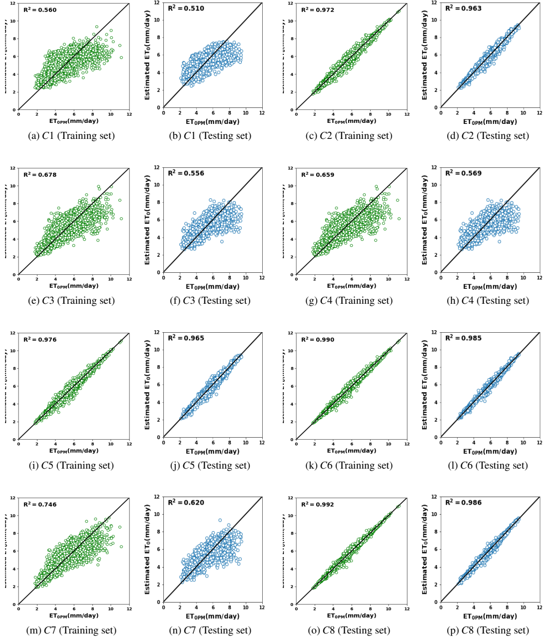
Figure 18: Scatter plots of estimated ET_0 against ET_{OPM} obtained for the training and testing sets of Tamaguri
