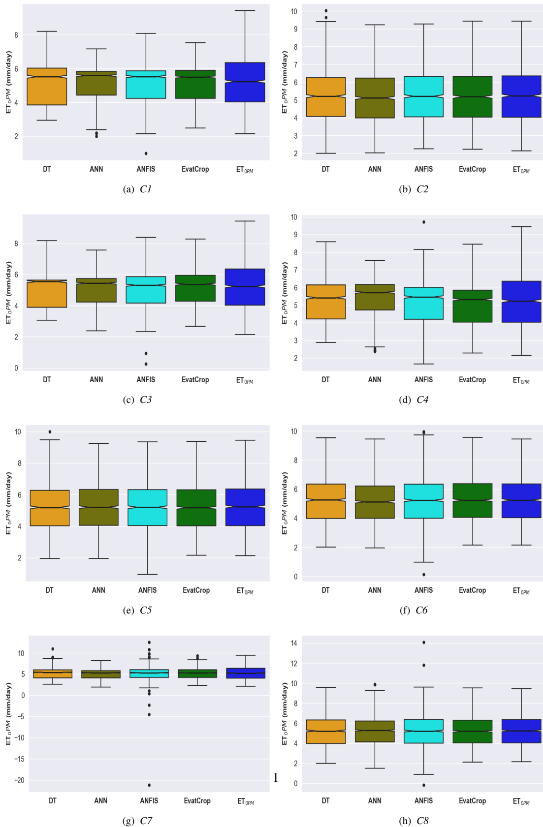
Figure 19: Boxplots for estimated ET_0 of DT, ANN, ANFIS, EvatCrop , and ET_{0PM} obtained for the testing set of Tamaguri
