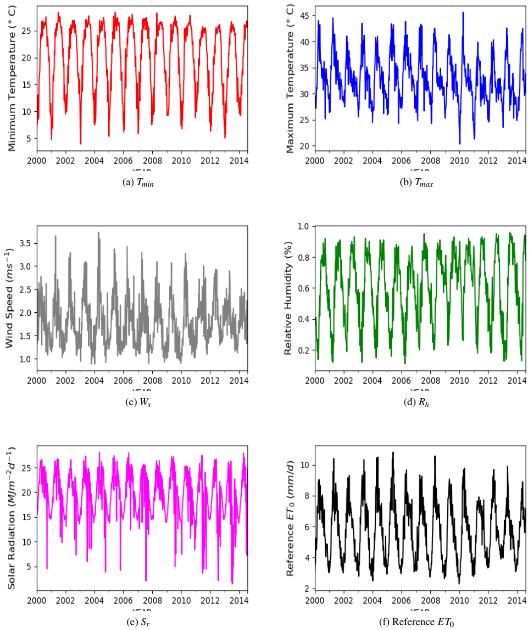
Figure 1: Time series plots for each of the input parameters and reference ET_0 for Berubari
