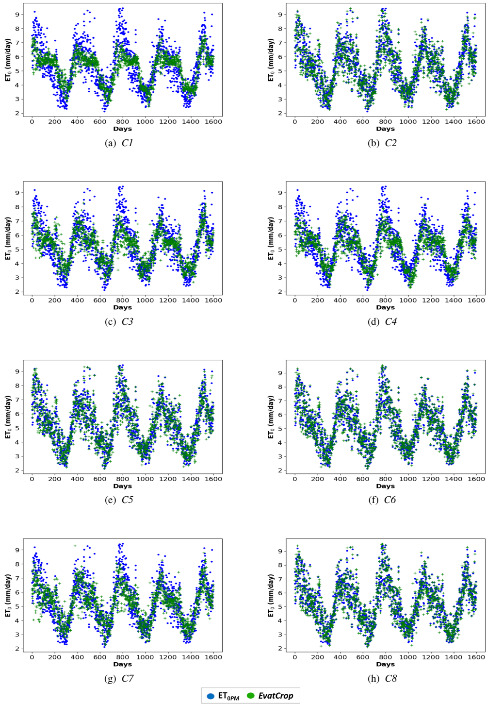
Figure 21: Distribution plots for estimated ET_0 of EvatCrop , and ET_{0PM} obtained for the testing set of Tamaguri
