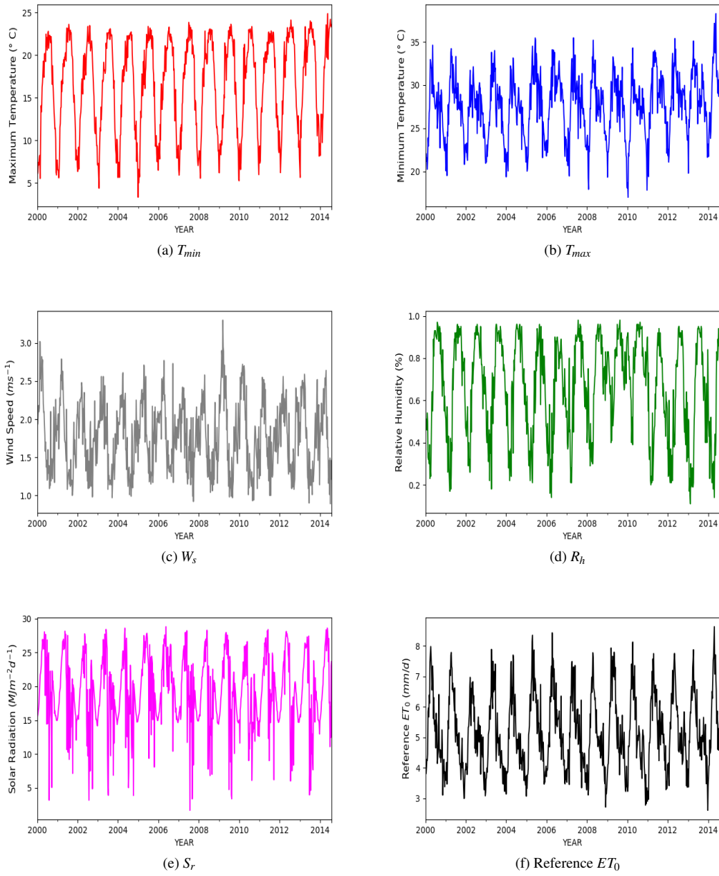
Figure 2: Time series plots for each of the input parameters and reference ET_0 for Jayanti
