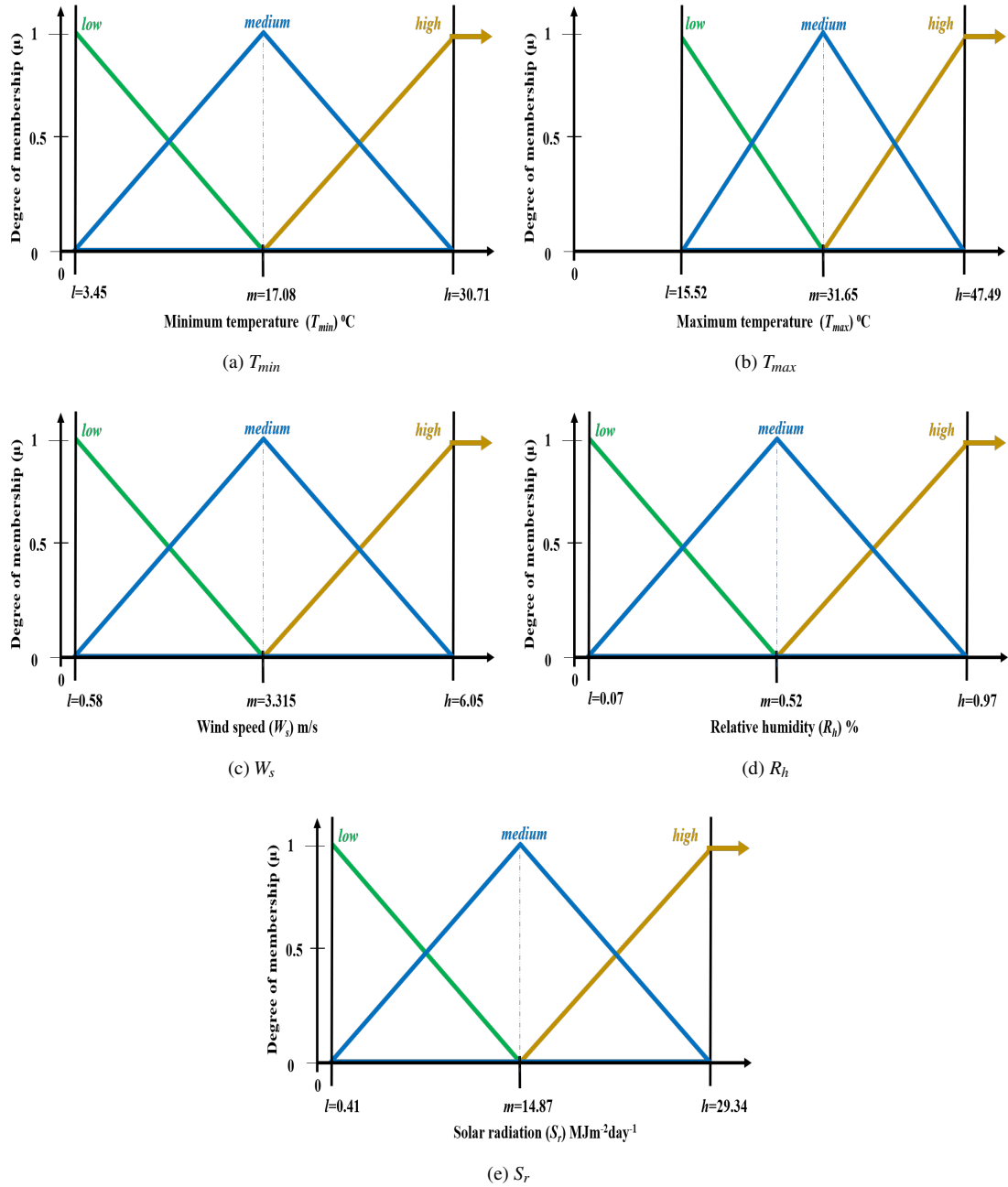
Figure 7: The shapes and range of values of fuzzy membership functions of each input parameter for Berubari
