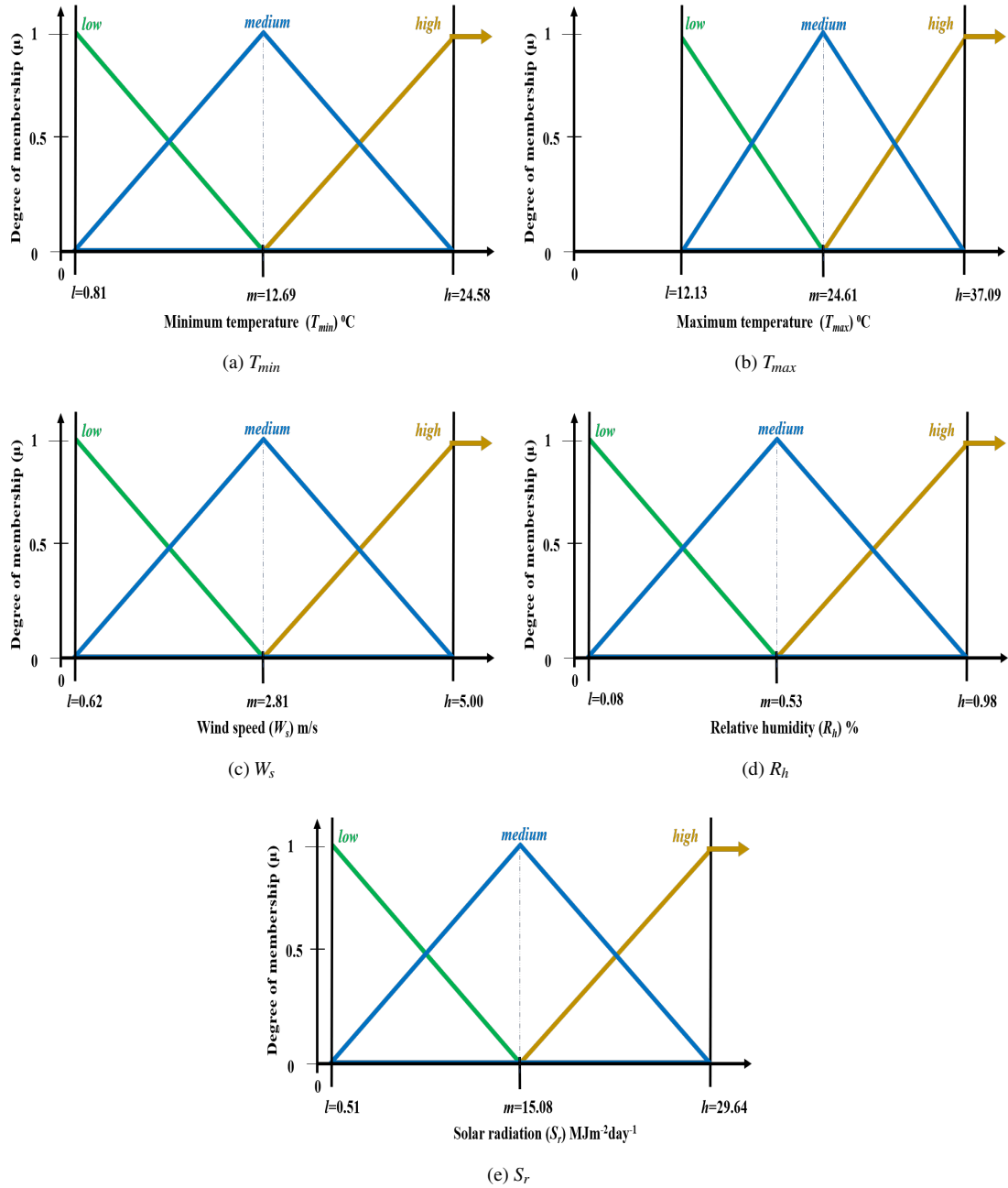
Figure 8: The shapes and range of values of fuzzy membership functions of each input parameter for Jayanti
