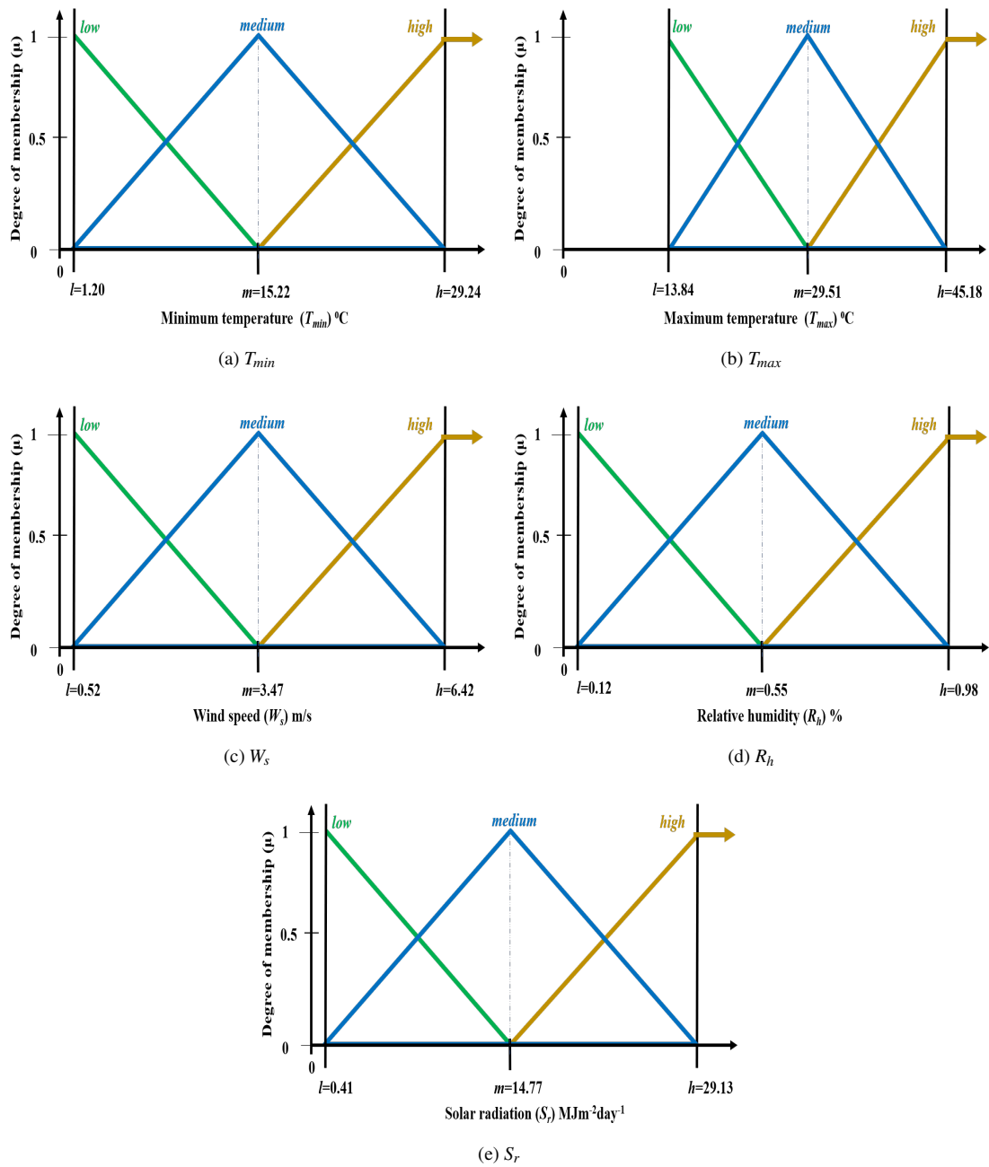
Figure 9: The shapes and range of values of fuzzy membership functions of each input parameter for Tam-aguri
