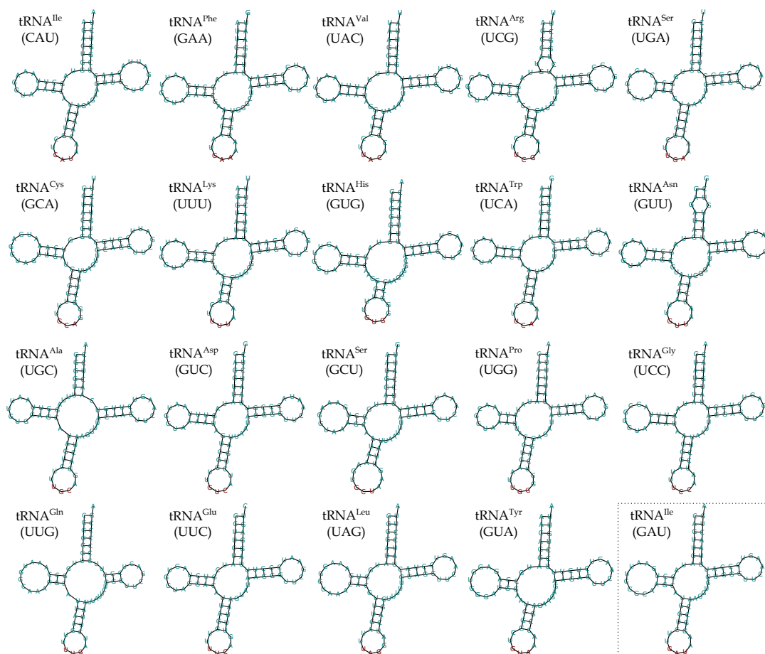
Figure S4. Transfer RNAs from the mitochondrial chromosome 1 (chrM1) and, in detail, putative mitochondrial chromosome 3 ( putative chrM3). Anticodon sequences in red.
