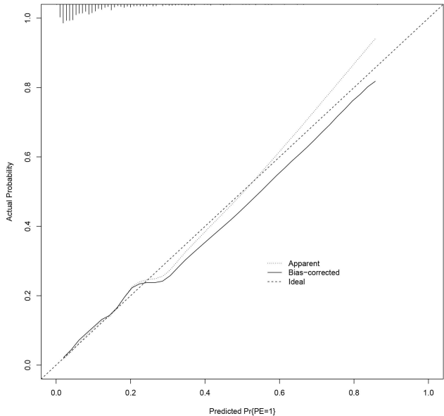
Fig. S1. The calibration plot for the nomogram
