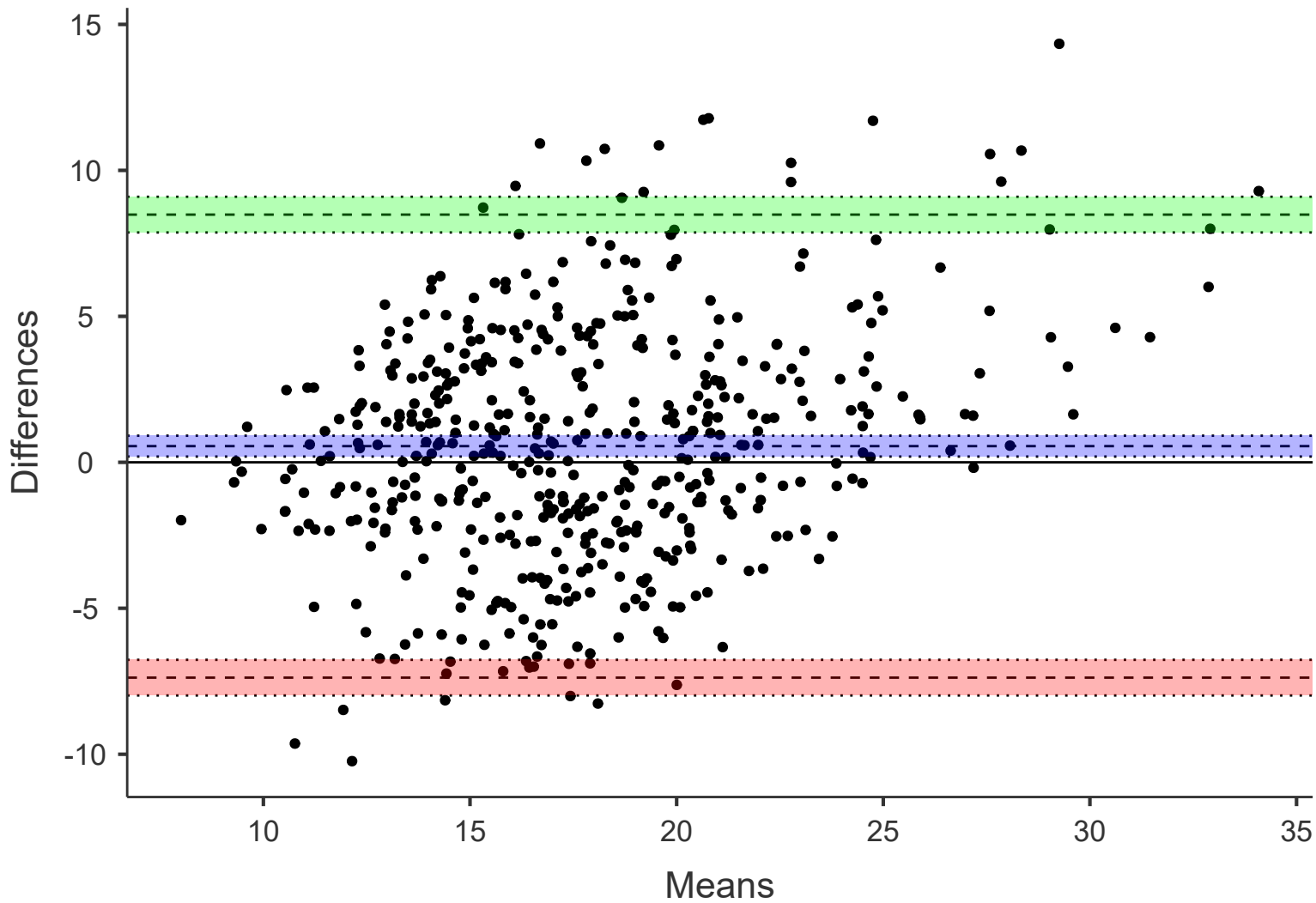
Bland-Altman plot
