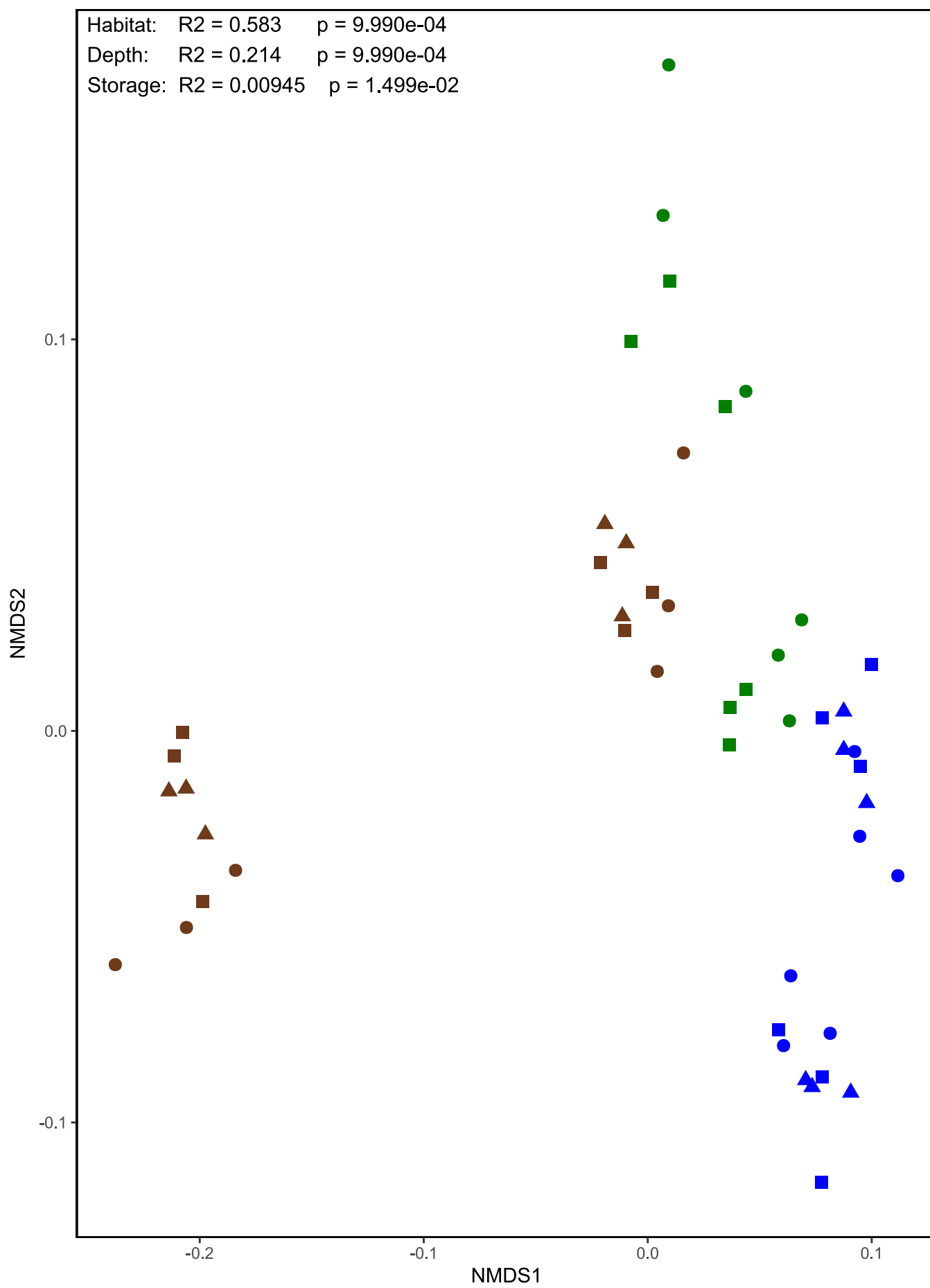
A) Bray-Curtis NMDS of Storage Methods
