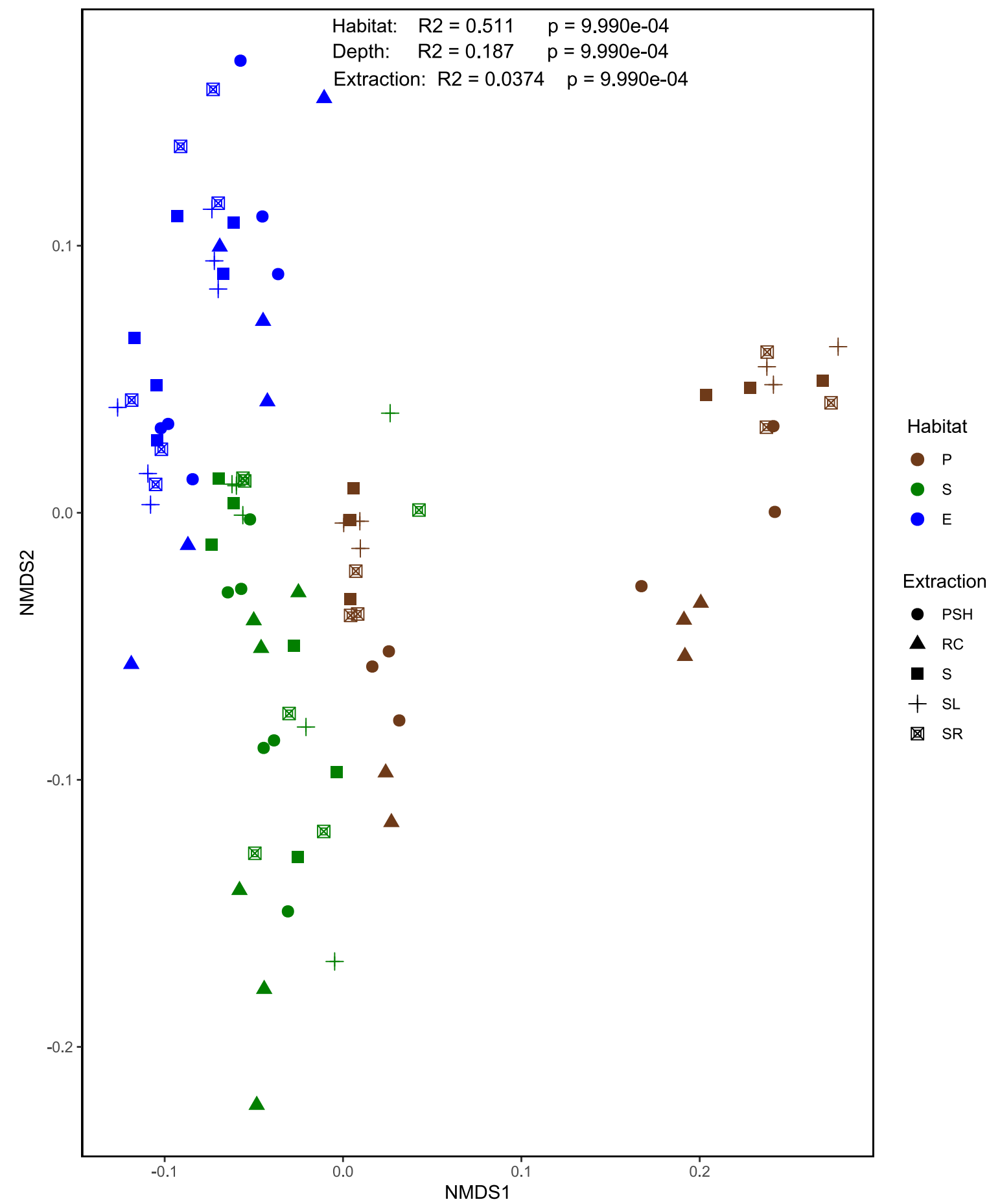
B) Bray-Curtis NMDS of Extraction Methods
