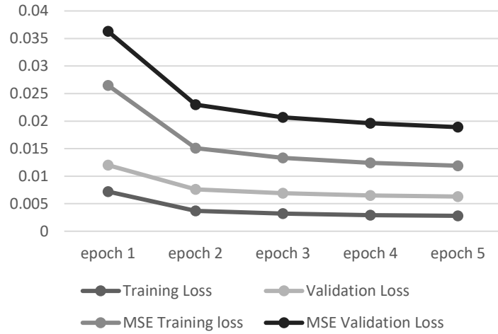
Wind Farm 1 - Stacked LSTM
