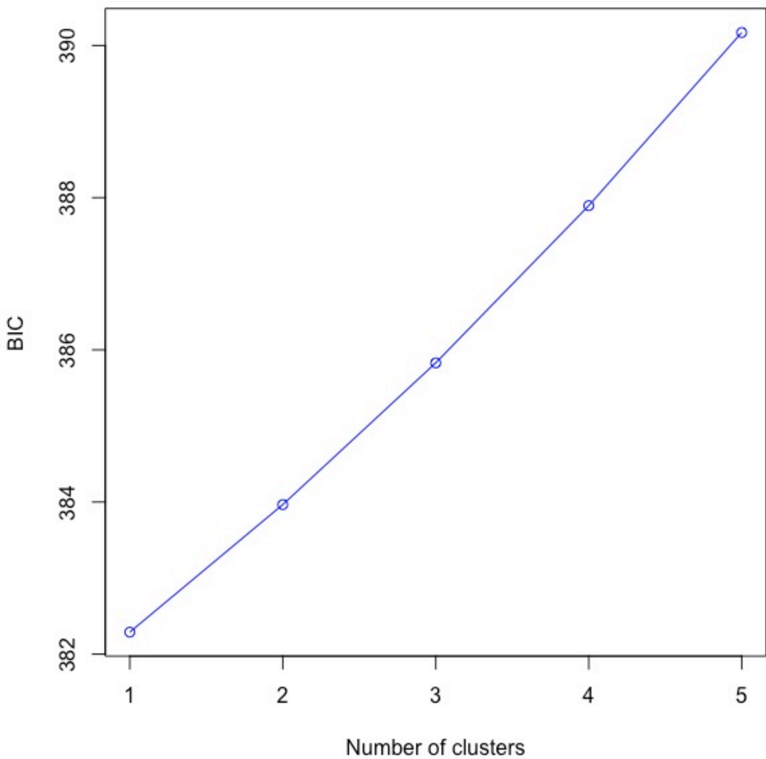
Value of BIC versus number of clusters
