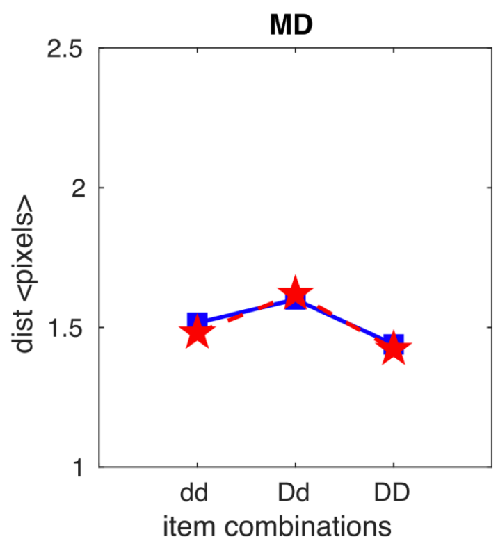
Figure S1. IL (top) and MD (bottom) of the target-in-the-middle trials for the simulation with movement onset scaling factor values as in Fig.6 (left) and Fig.7 (right).
