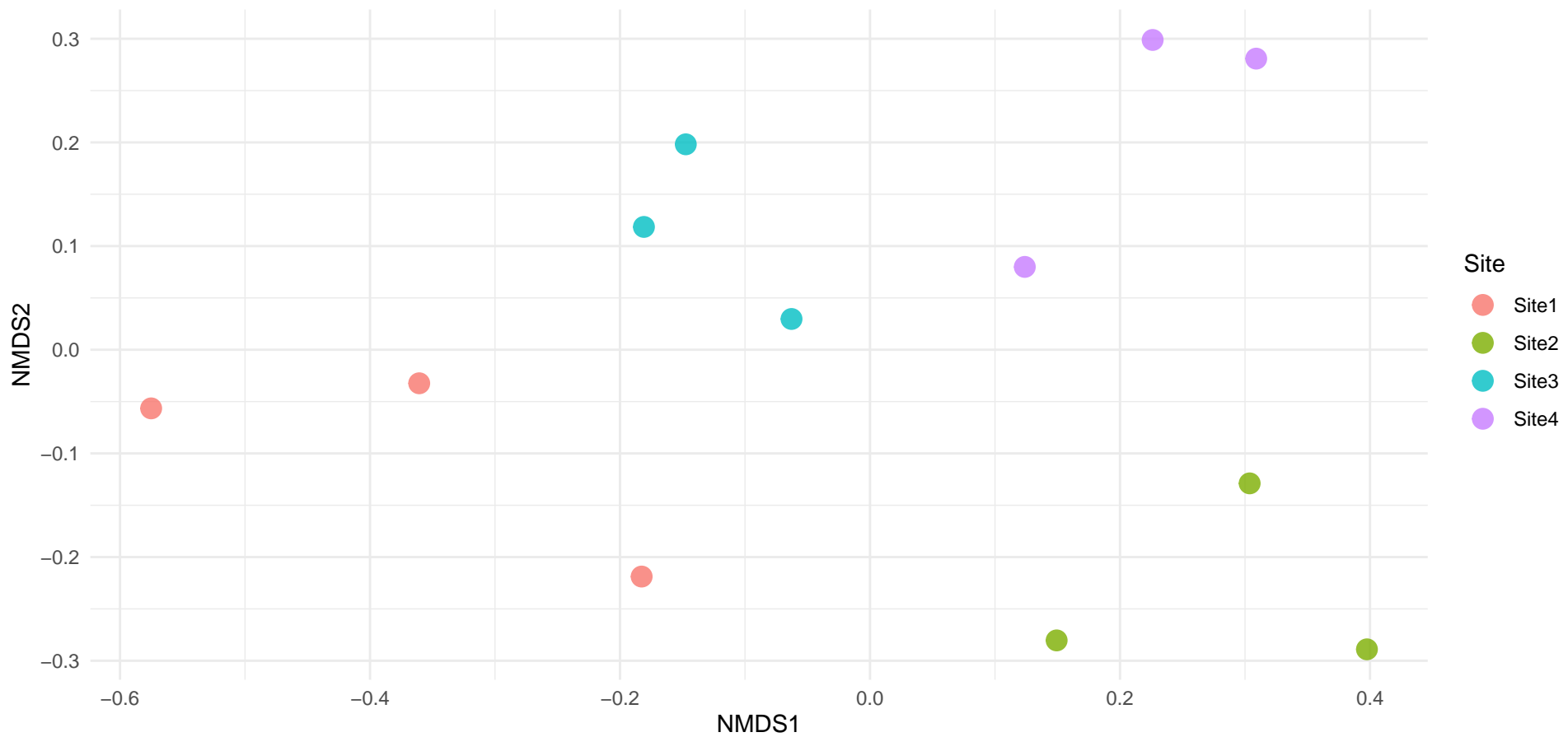
NMDS based on Jaccard distance
