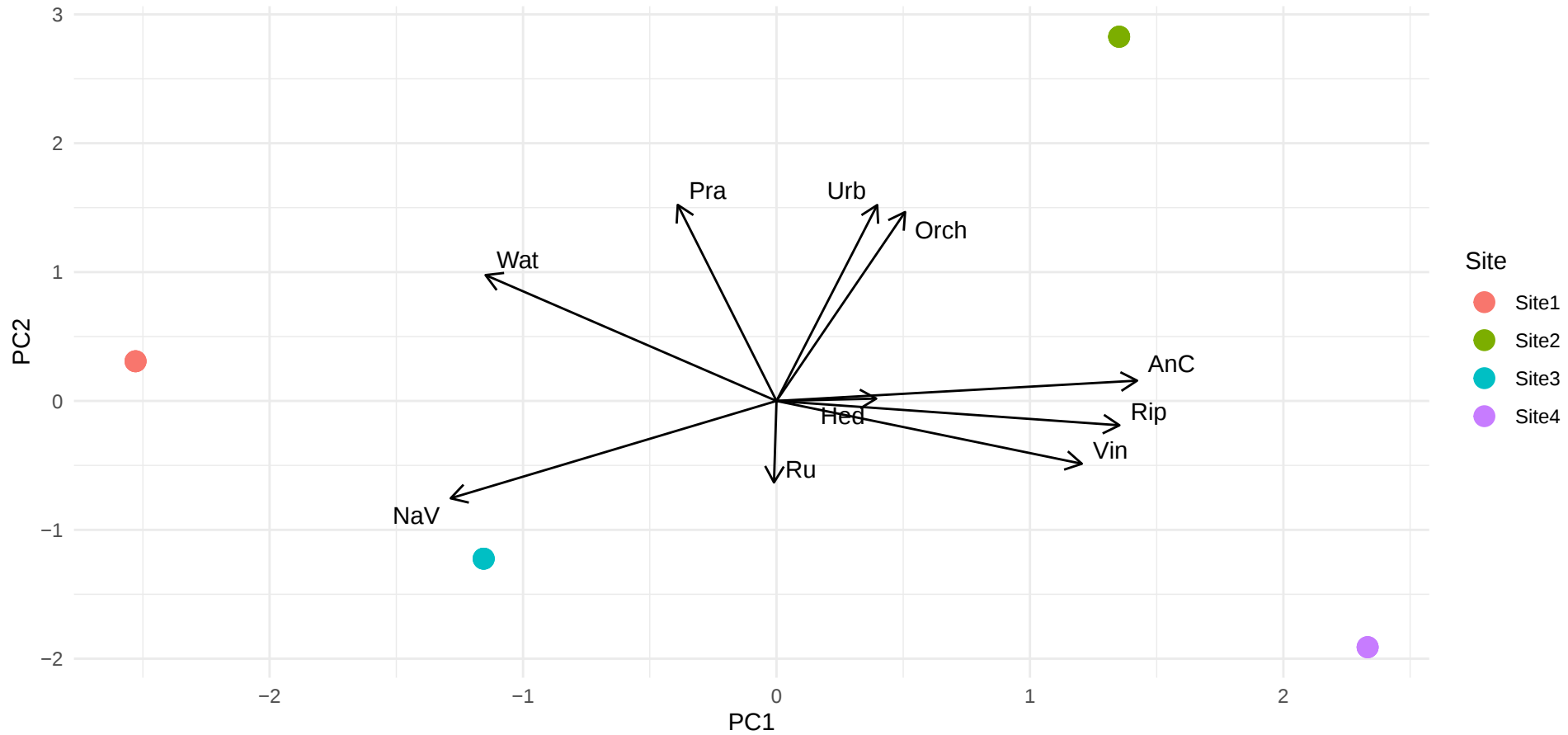
PCA Biplot of Site Characteristics
