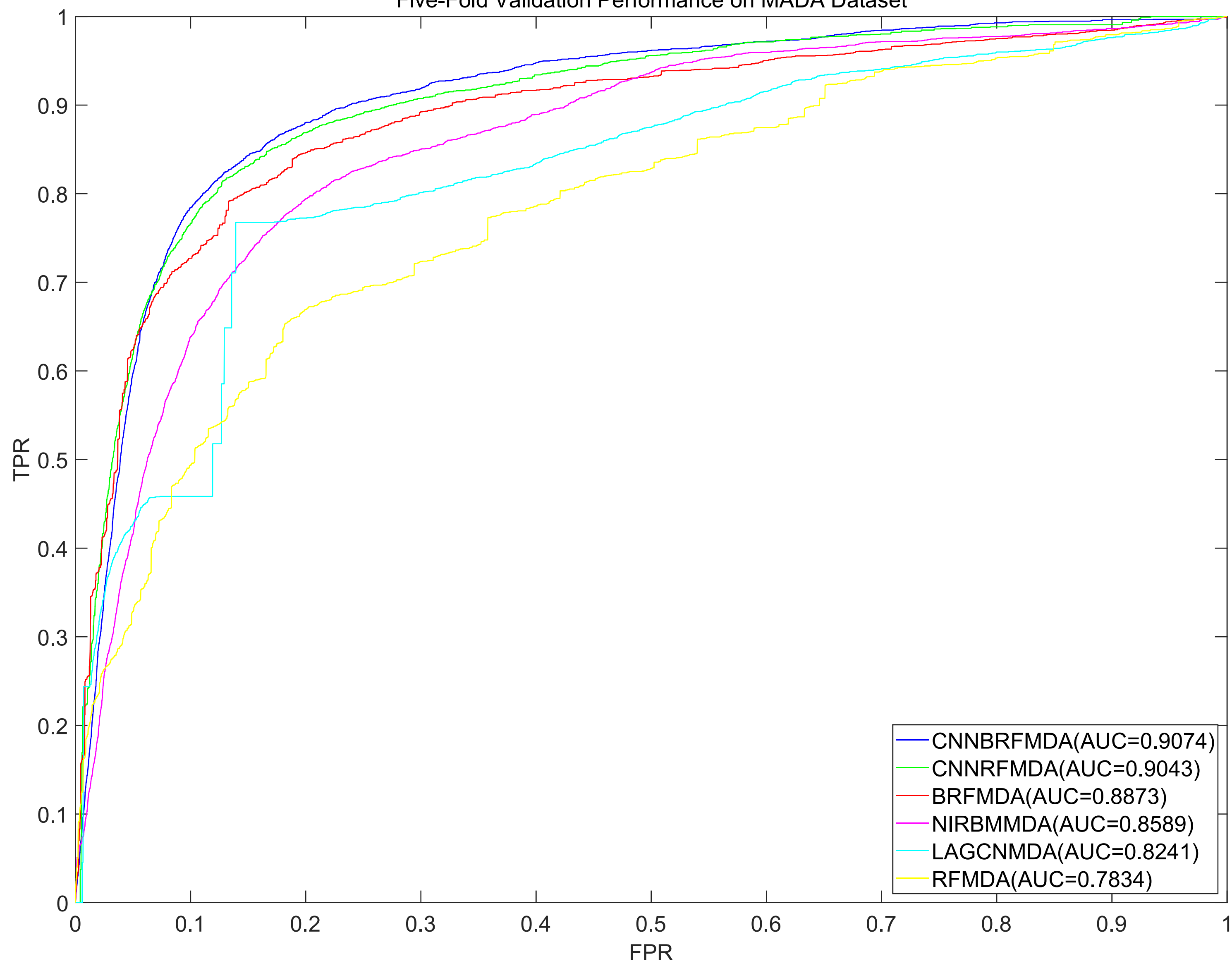
Five-Fold Validation Performance on MADA Dataset
