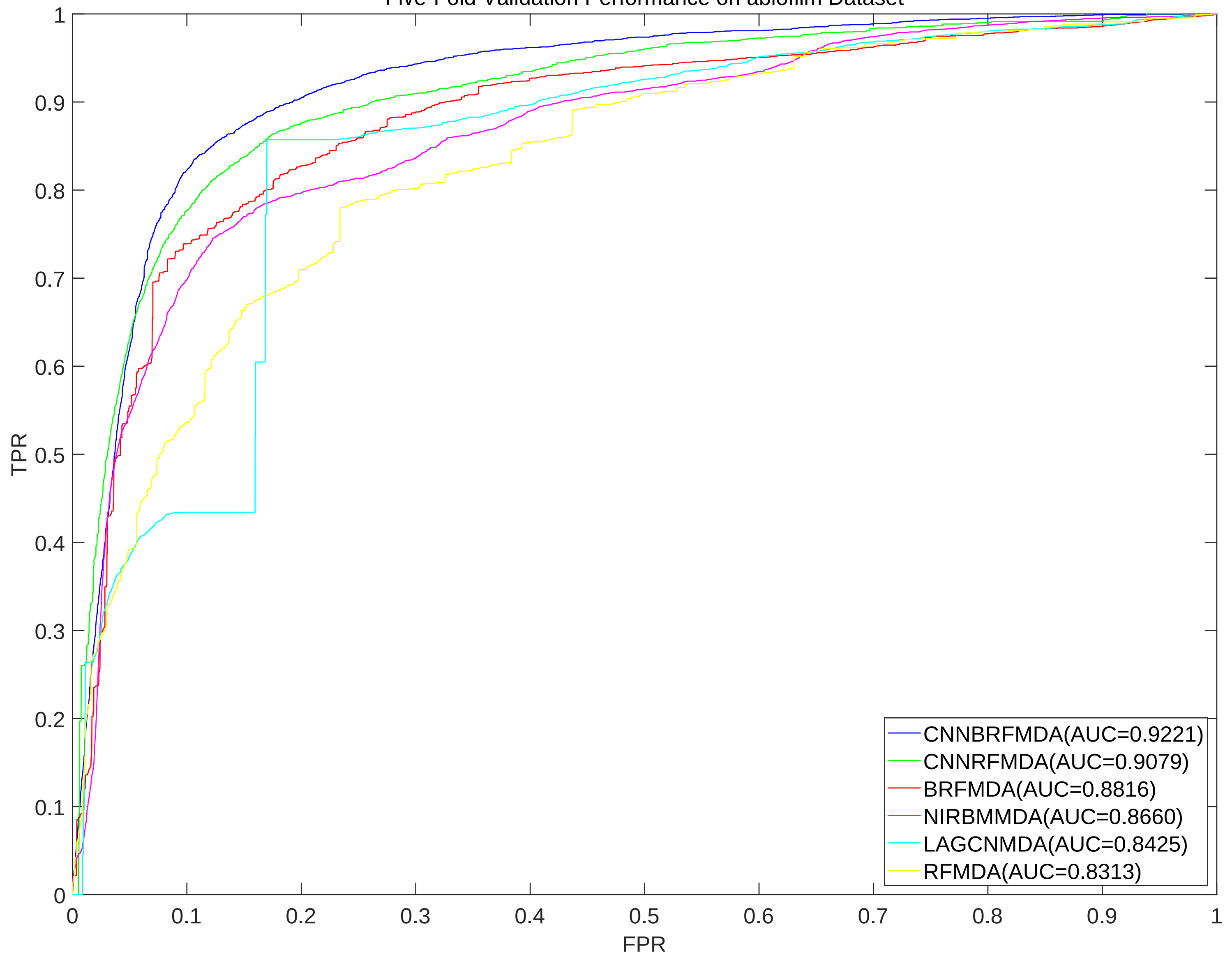
Five-Fold Validation Performance on abiofilm Dataset
