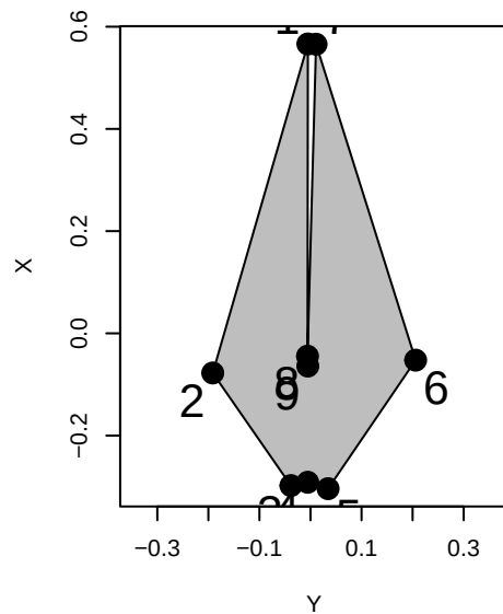
Cephalorhynchus_eutropia
