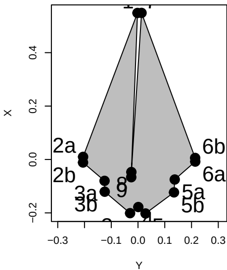
Peponocephala_electra
