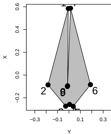
Delphinus_delphis
