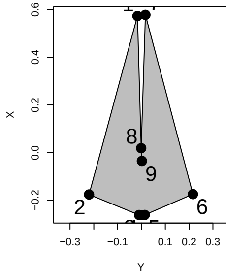
Balaena mysticetus
