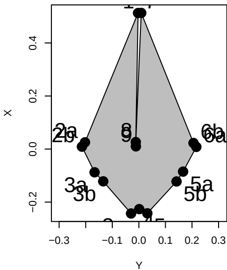
Phocoena_phocoena
