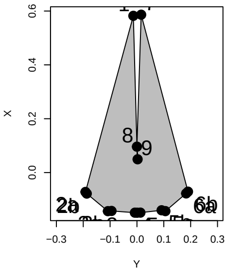
Balaena mysticetus
