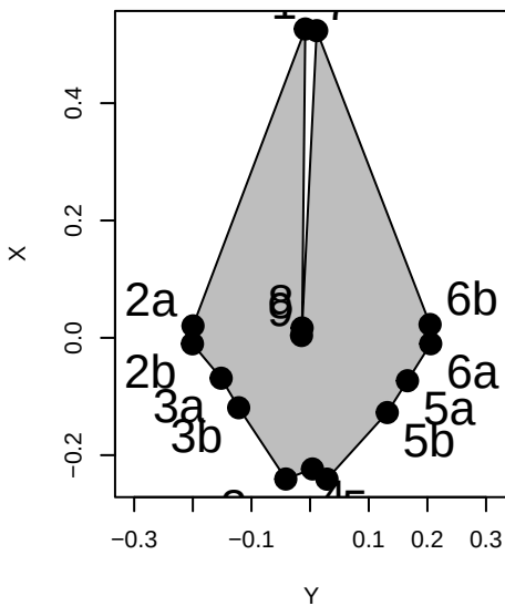
Cephalorhynchus_heavisidii
