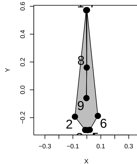
Caperea_marginata
