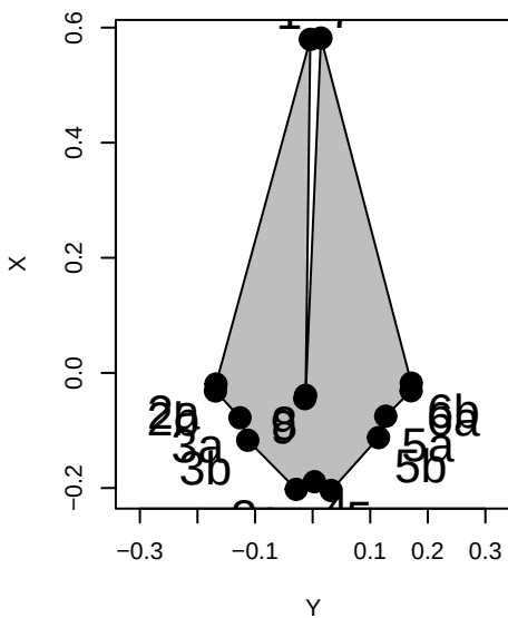
Delphinus_delphis
