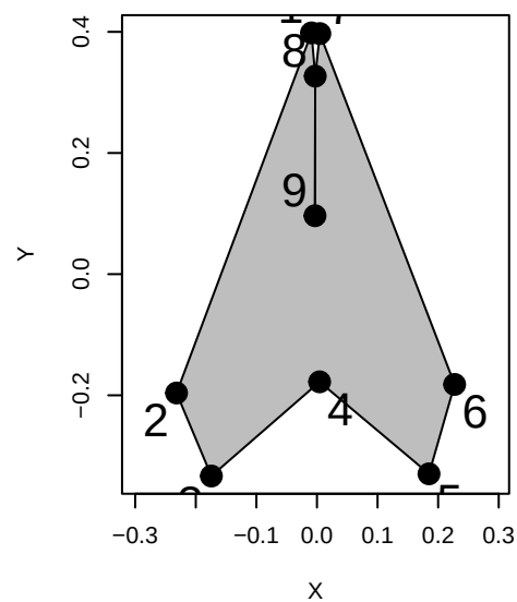
Balaena mysticetus
