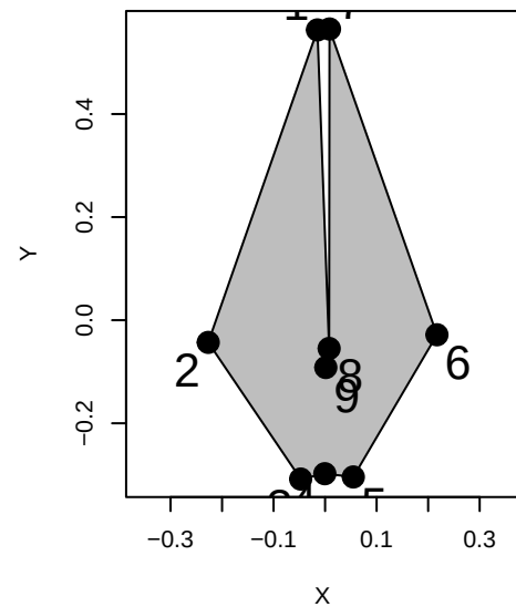
Phocoena_dioptrica
