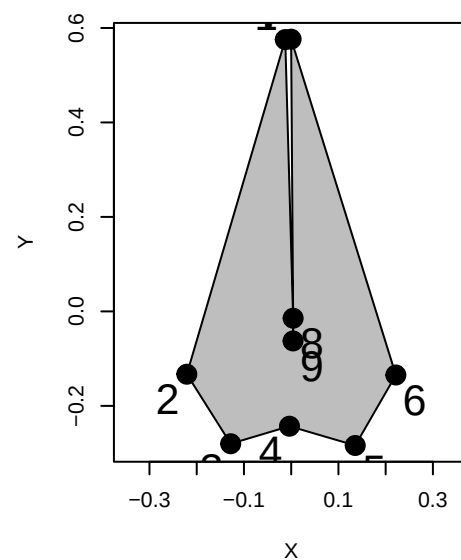
Peponocephala_electra
