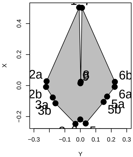
Phocoena_dioptrica
