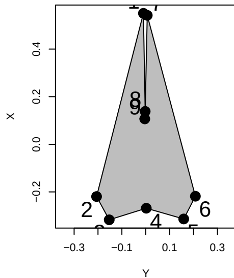
Caperea_marginata
