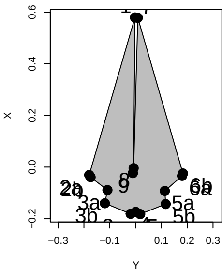
Mesoplodon_europaeus
