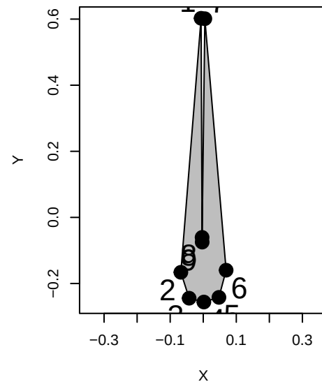
Cephalorhynchus_heavisidii
