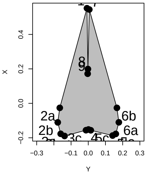
Caperea_marginata
