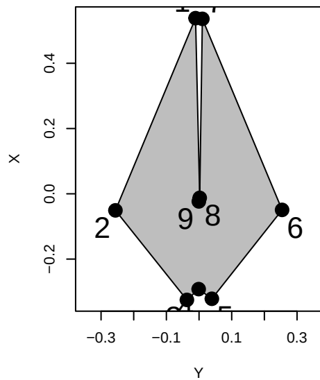
Phocoena_dioptrica
