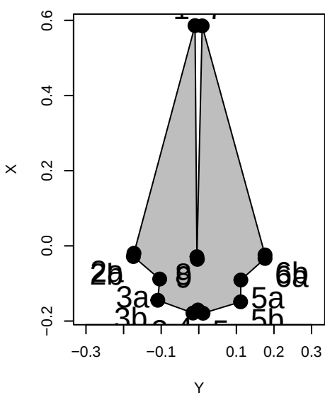
Tasmacetus_shepherdi
