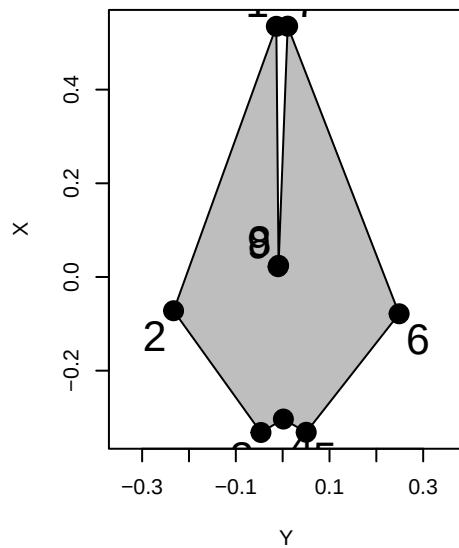
Phocoena spinipinnis
