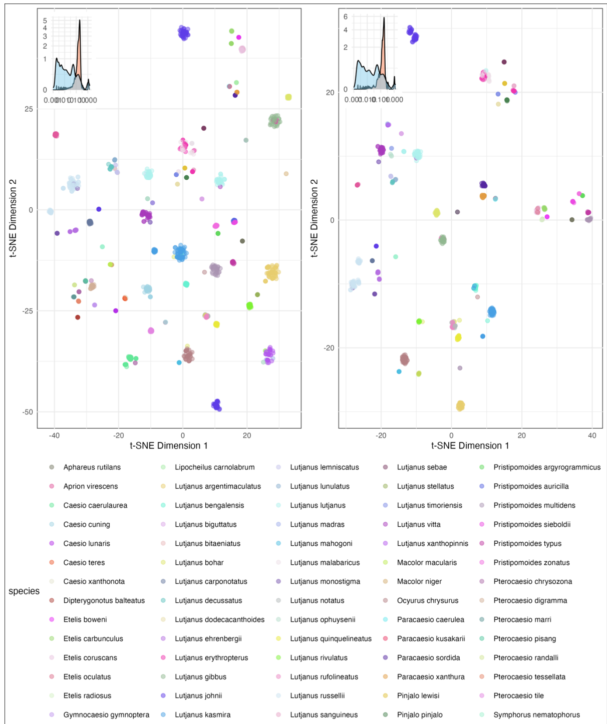
Supplementary figure 1. t-SNE clustering of sequences from NCBI (left) and BOLD (right) for Lutjanidae species.
