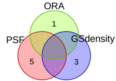
spatialGE_psf_3
