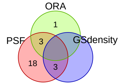
spatialGE_psf_11
