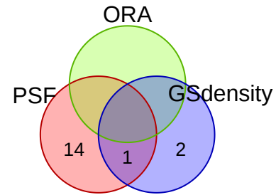
spatialGE_psf_10
