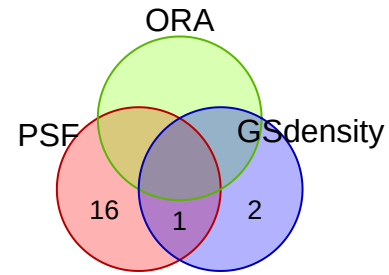
spatialGE_psf_2
