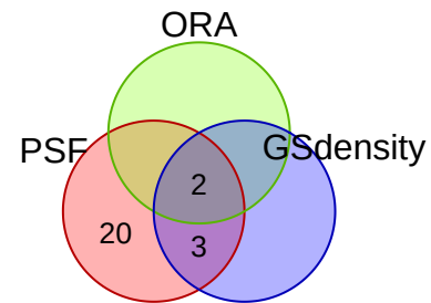
vesalius_exp_10
