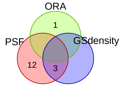
spatialGE_psf_1
