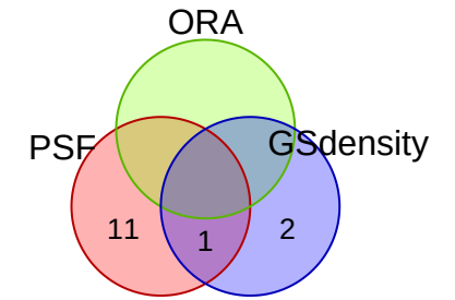
spatialGE_psf_4
