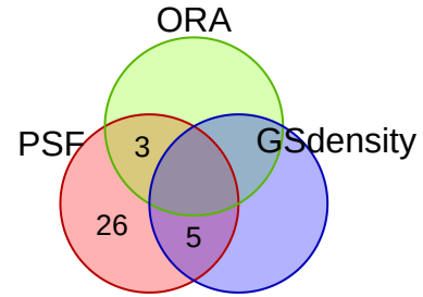
spatialGE_psf_5
