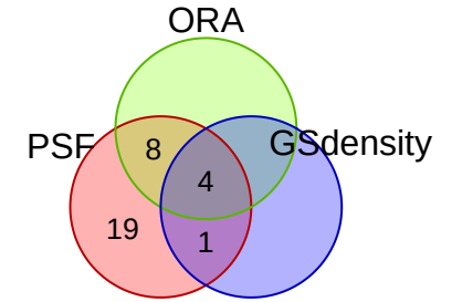
spatialGE_psf_8
