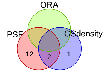
spatialGE_psf_8
