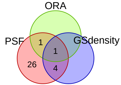
spatialGE_psf_6
