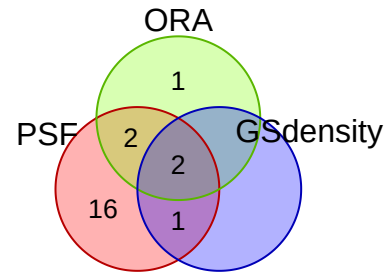
spatialGE_psf_9
