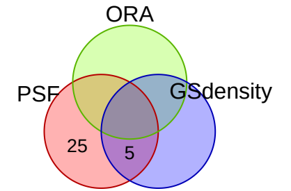
spatialGE_psf_4
