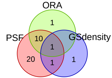
spatialGE_psf_7
