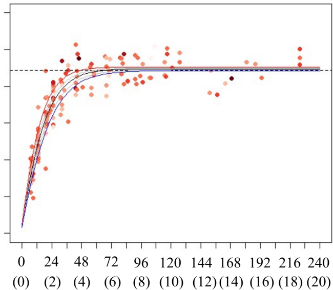
Model 1 ( \Delta AIC=1.89 )
