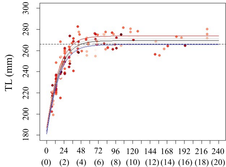
Model 3 ( \Delta AIC=1.87 )
