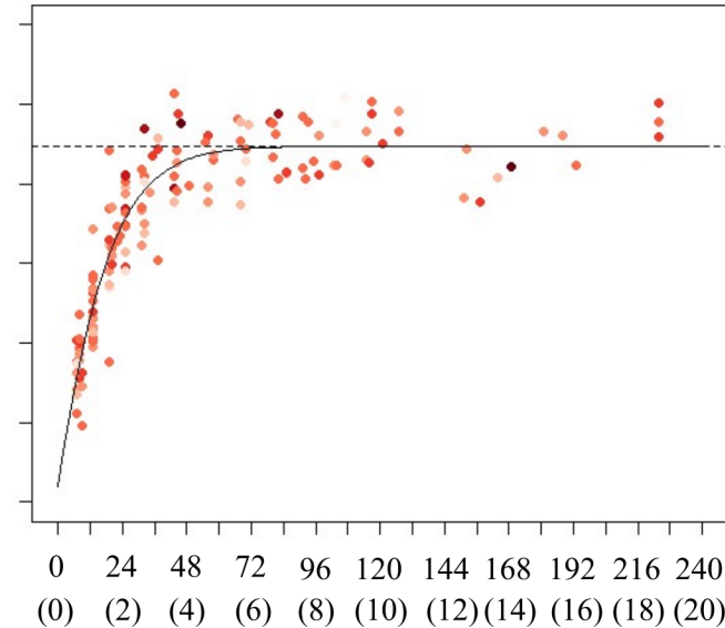
Model 4 ( \Delta AIC=3.21 )
