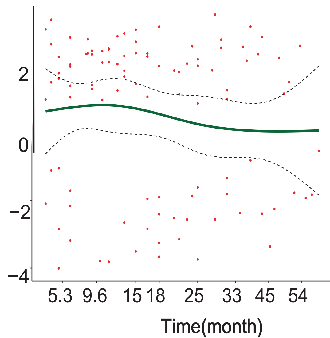
Schoenfeld Individual Test p: 0.0202
