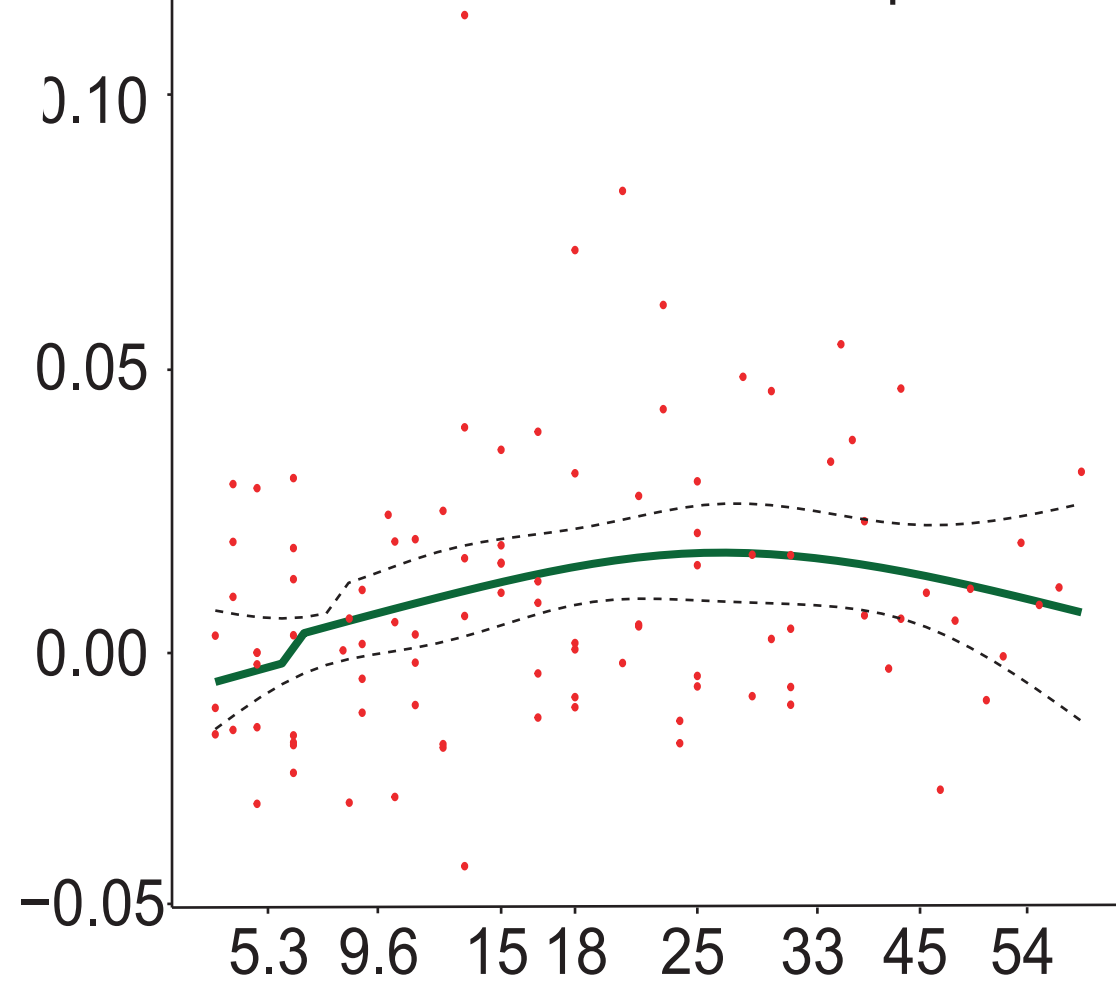
Schoenfeld Individual Test p: 0.0162
