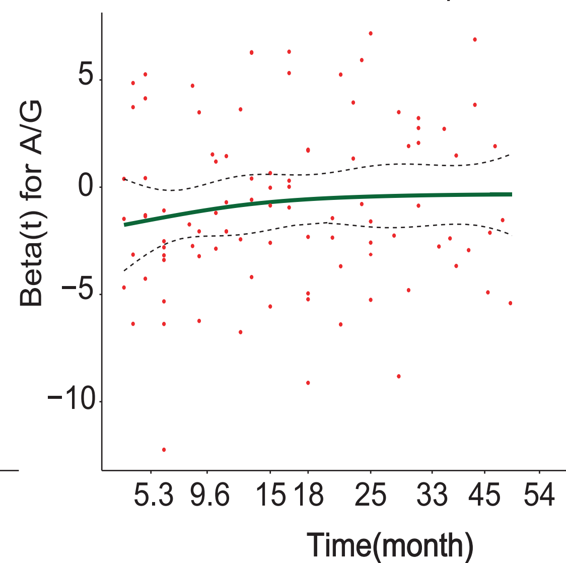
Schoenfeld Individual Test p: 0.4351
