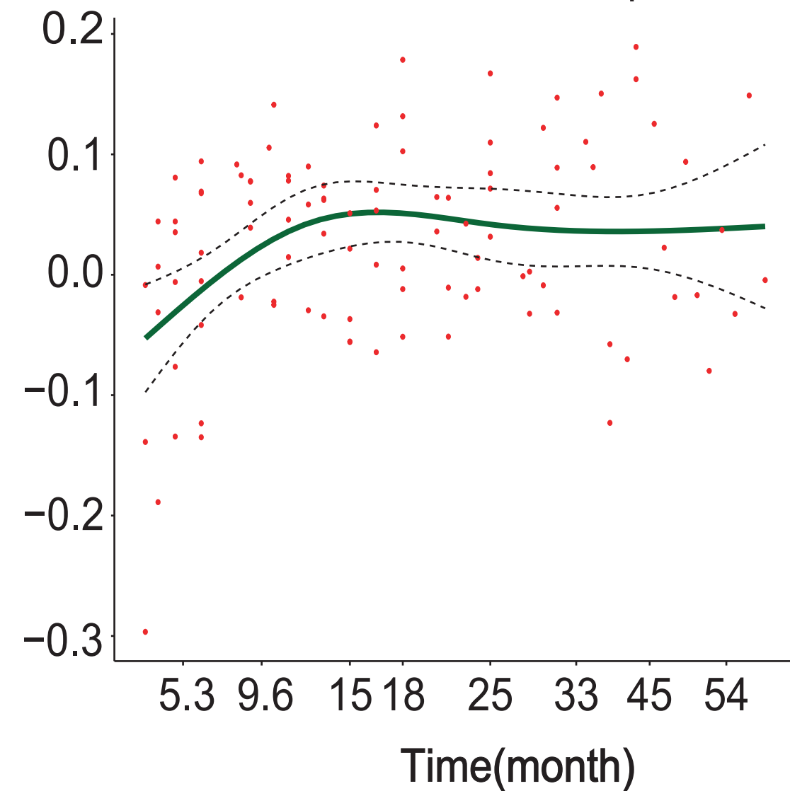
Schoenfeld Individual Test p: 0.0202
