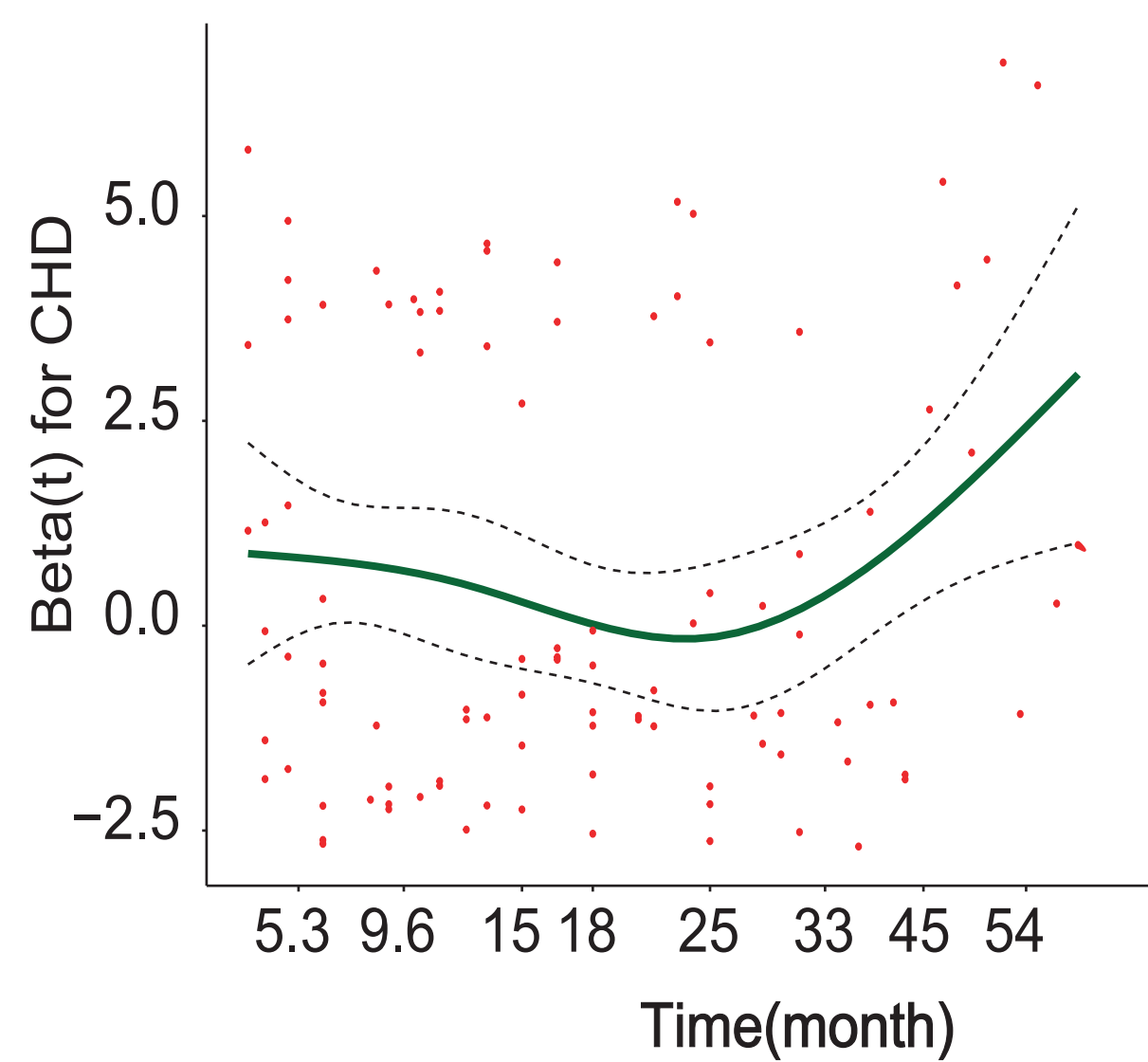
Schoenfeld Individual Test p: 0.4689
