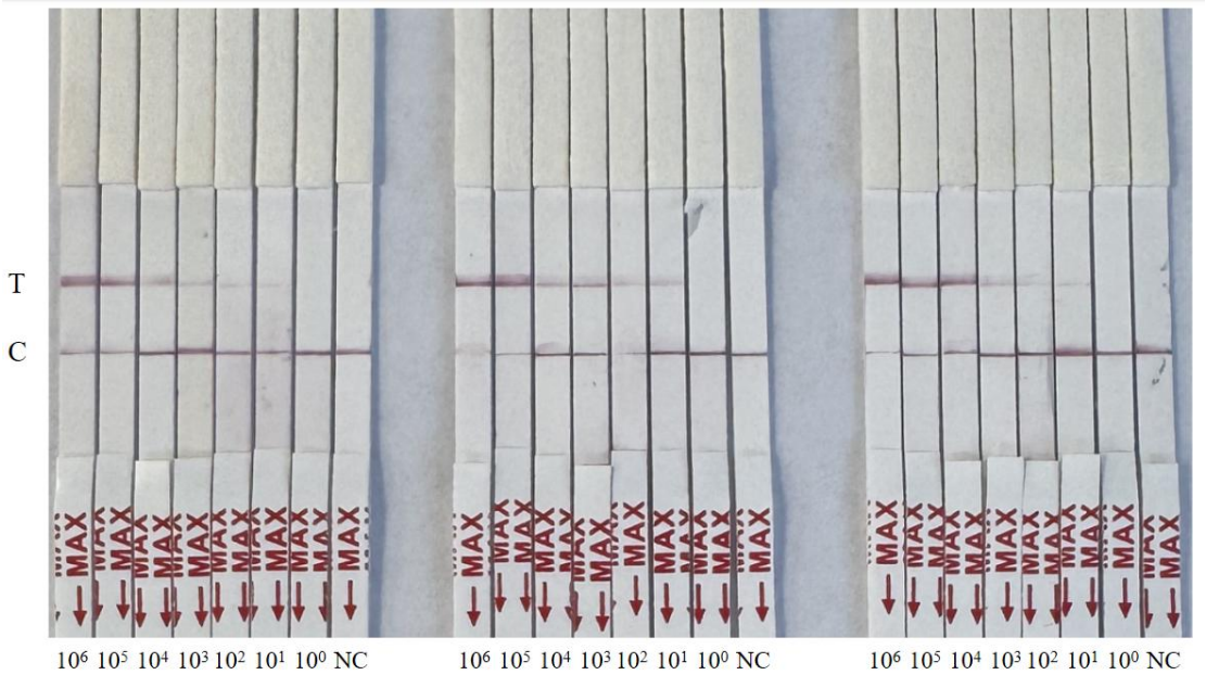
Figure 1S:Repeatable experiment of RT-RPA-CRISPR/Cas12a-LFD sensitivity.C:control line, T:test line, NC:negative control.
