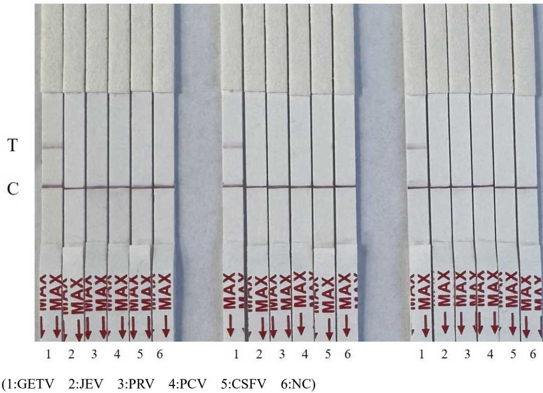
Figure 2S:Repeatable experiment of RT-RPA-CRISPR/Cas12a-LFD specificity.C:control line, T:test line, NC:negative control
