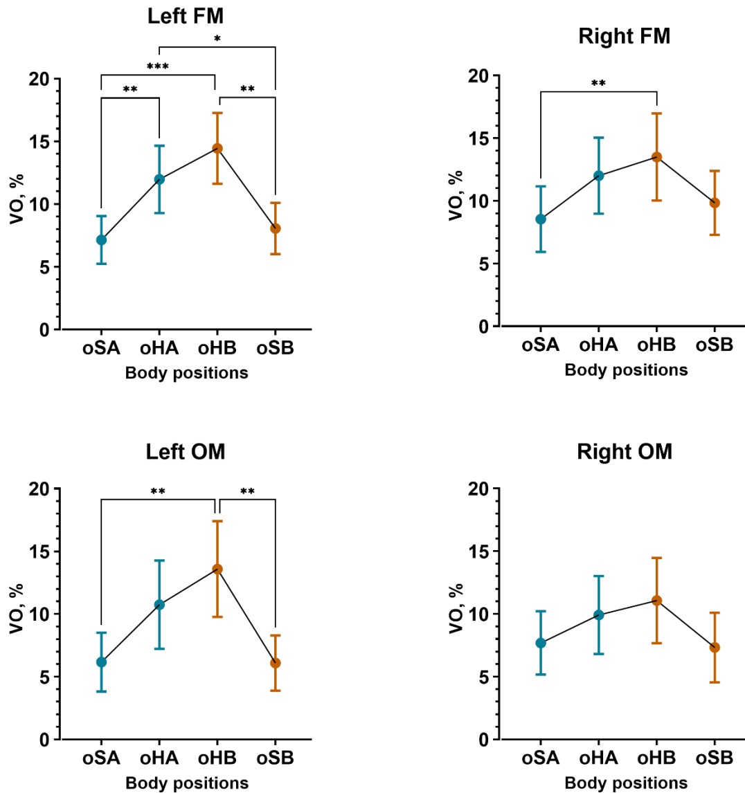
Supplemental Figure 15. Postural changes of VO among male participants during Test 2 (n = 16). The graphs show data from 4 REG leads: left and right fronto-mastoid (FM), left and right occipito-mastoid (OM) for sitting and supine positions. The graphs show confidence intervals with means represented by circle-shaped points, and medians depicted as rhomb-shaped points. Additionally, points and intervals are highlighted by different colors to distinguish between first sitting (oSA) and supine (oHA) positions and second sitting (oSB) and supine (oHB) positions. A one-way repeated measures ANOVA summary for statistically significant results: left FM ( F(1.697, 25.46) = 16.03, p < 0.0001 ), right FM ( F(3, 45) = 4.812, p = 0.0054 ), left OM ( F(2.073, 31.10) = 9.858, p = 0.0004 ). “*” – p < 0.05 , “**” – p < 0.01 , “***” – p < 0.001 .
