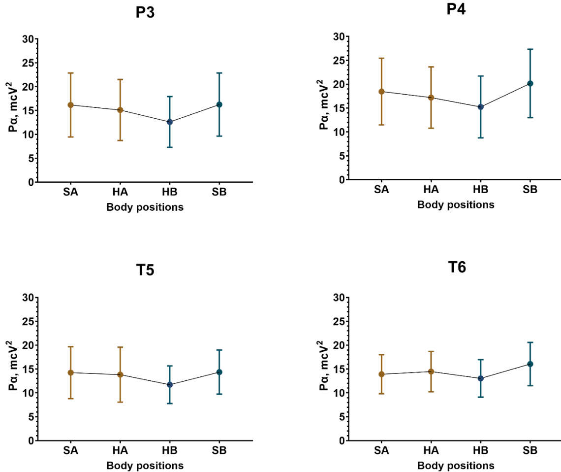
Supplementary Figure 38. Postural changes of alpha spectral power ( P_{\alpha} ) calculated for P3, P4, T5 and T6 electrodes among female participants during Test 1 ( n = 16 ). The graphs show confidence intervals with means represented by circle-shaped points. Additionally, points and intervals are highlighted by different colors to distinguish between first sitting (SA) and first 2 minutes of supine (HA) position and second sitting (SB) and last 2 minutes of supine (HB) position.
