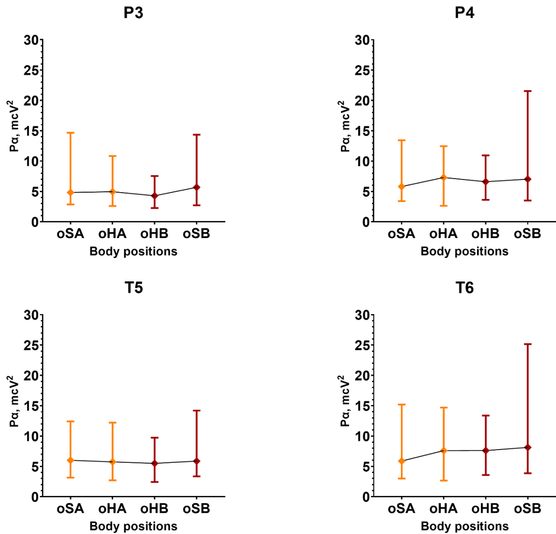
Supplemental Figure 49. Postural changes of alpha spectral power ( P_{\alpha} ) calculated for P3, P4, T5 and T6 electrodes among male participants during Test 2 ( n = 16 ). The graphs show confidence intervals with medians depicted as rhomb-shaped points. Additionally, points and intervals are highlighted by different colors to distinguish between first sitting (oSA) and supine (oHA) positions and second sitting (oSB) and supine (oHB) positions.
