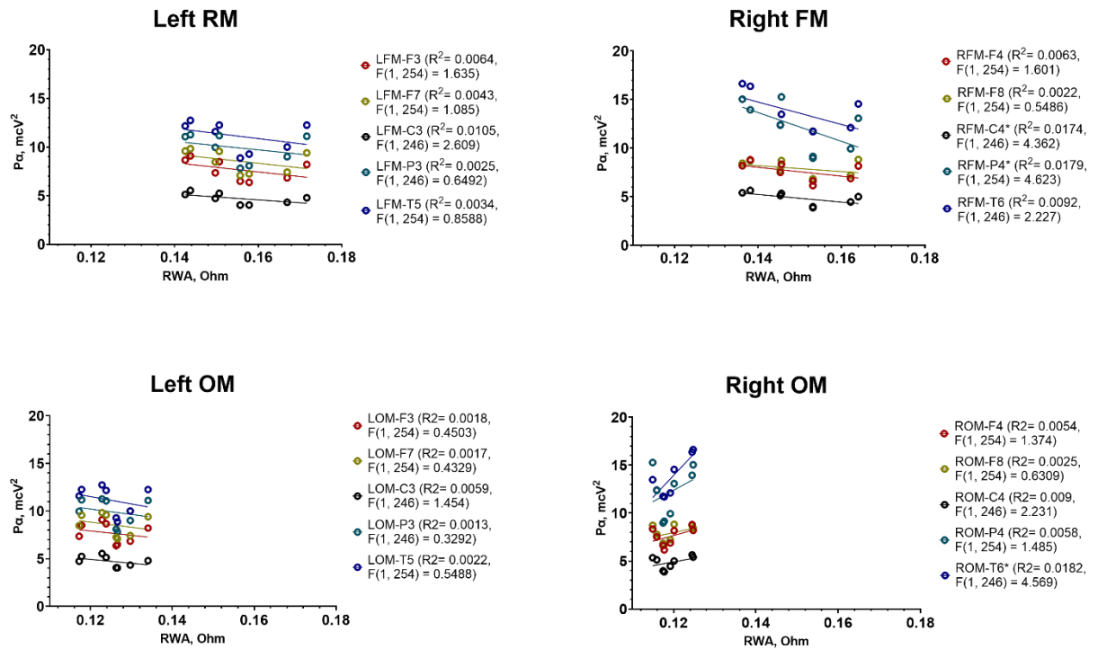
Supplemental Figure 64. Simple linear regression graphs showing estimated relationship between RWA and P\alpha in all 4 REG leads and several corresponding EEG electrodes among all participants in Test 2 ( n = 8 ). Each point of certain color represents estimated relationship between RWA and P\alpha in the corresponding pair of REG lead and EEG electrode, for example, left FM and F3 (LFM-F3), right OM and C4 (RFM-C4), etc. The lines indicate the general trend of the relationship
