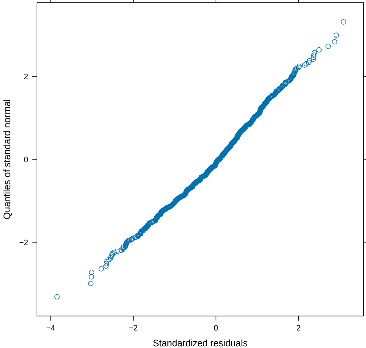
Q-Q Plot of Residuals
