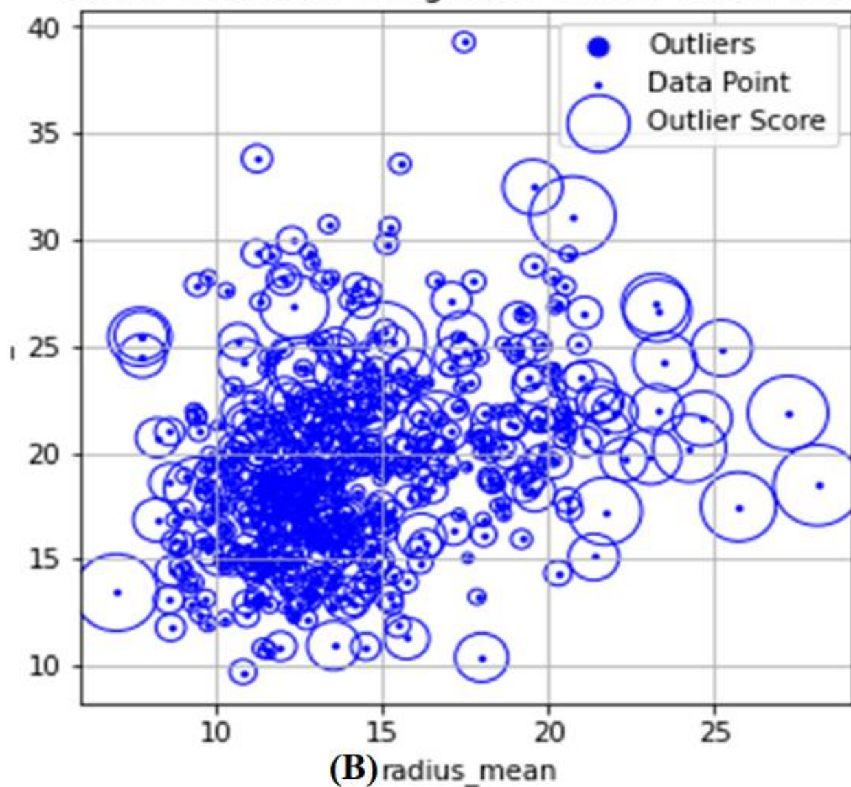
Outlier Detection using Local Outlier Factor (LOF)
