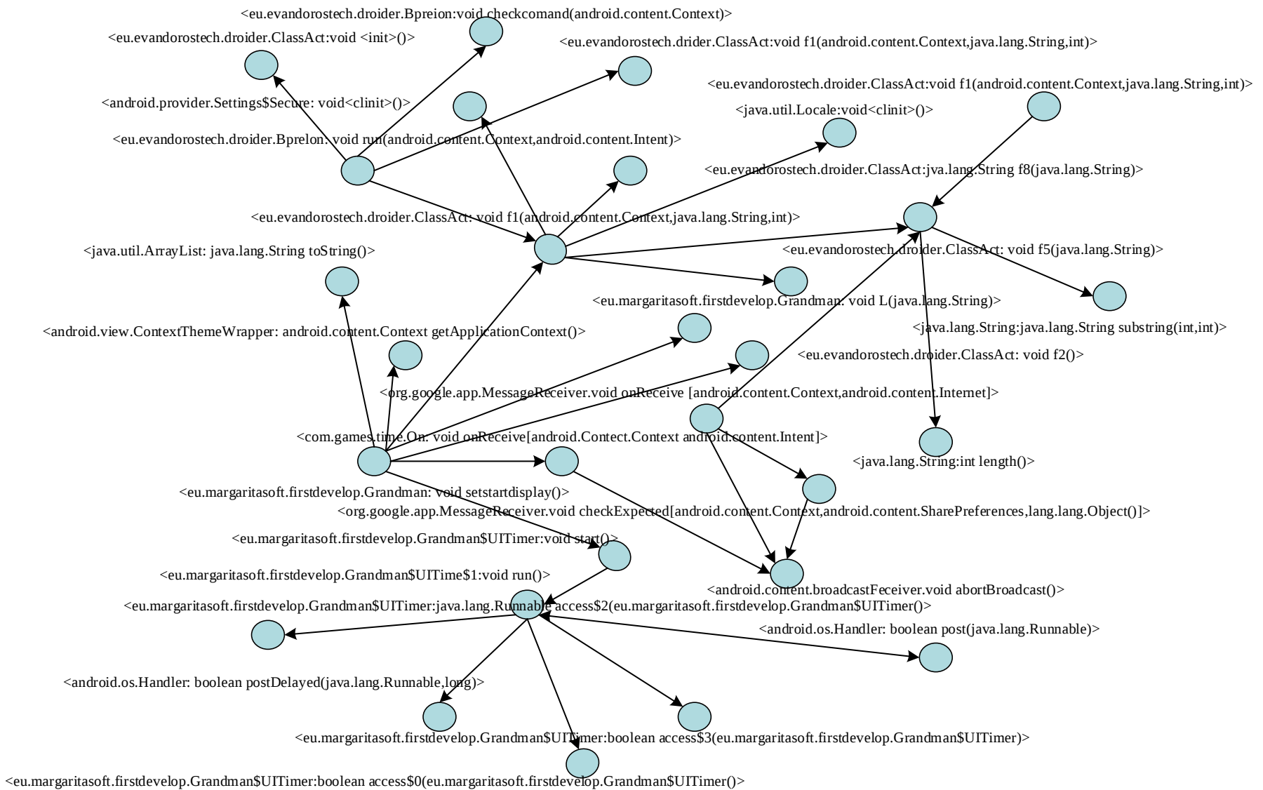
(a) function call graph before optimization
