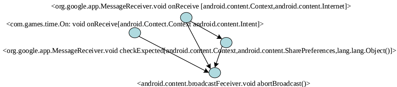
(b) Optimized function call graph
