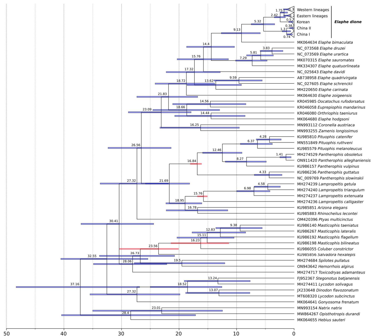
Figure S1. Time-calibrated tree with all outgroups shown. Numbers with branches indicate mean estimated node ages (in millions of years) and, together with blue bars, 95% highest posterior densities of the estimated node ages. Calibration points are highlighted with pink bars.
