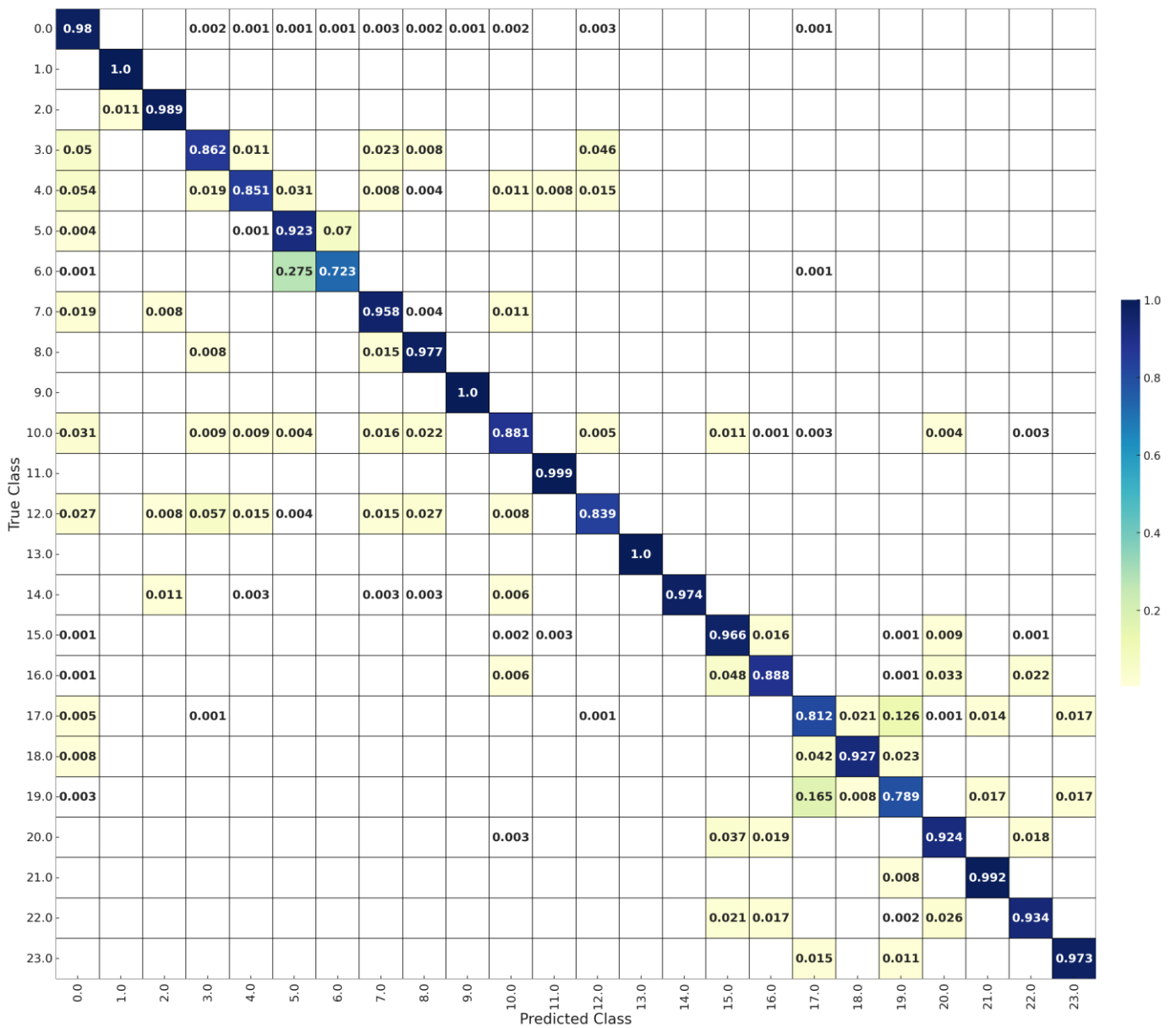
(C) Decision Tree Confusion Matrix
