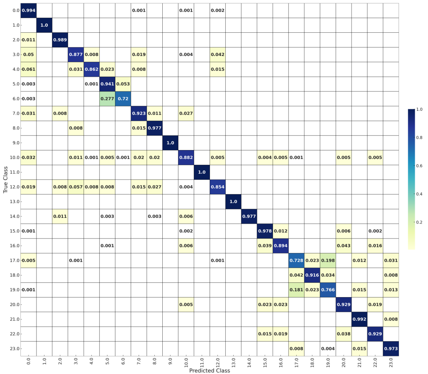
(B) Random Forest Confusion Matrix
